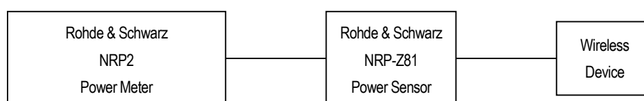
Figure 10.4 Power Measurement Setup
