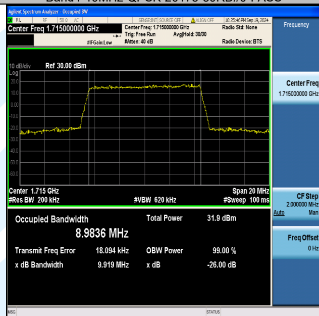
Band4-10MHz-16QAM-20000-50RB#0-PASS
