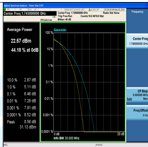
Band66-20MHz-16QAM-132322-100RB#0-PASS
