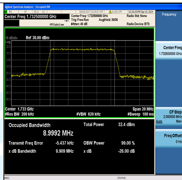
Band4-10MHz-QPSK-20175-50RB#0-PASS
