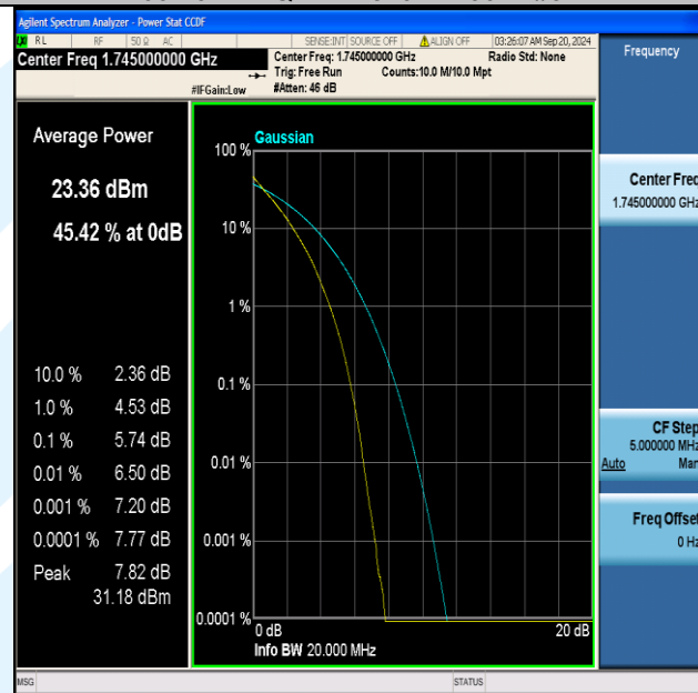
Band66-20MHz-QPSK-132322-100RB#0-PASS
