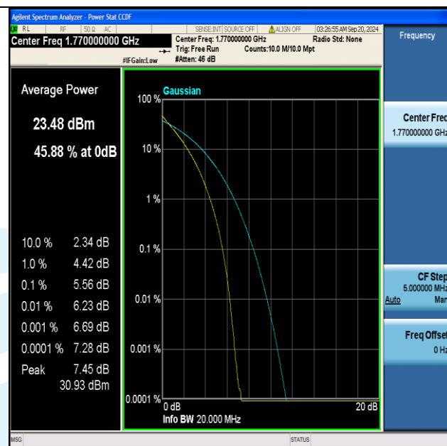
Band66-20MHz-QPSK-132572-100RB#0-PASS
