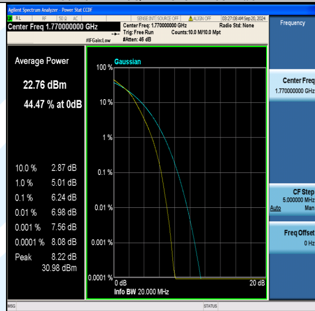
Band66-20MHz-16QAM-132572-100RB#0-PASS
