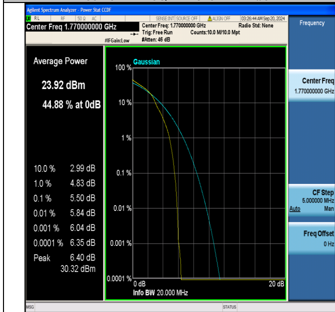
Band66-20MHz-16QAM-132572-1RB#0-PASS
