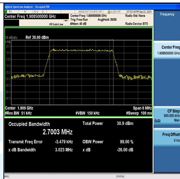
Band2-3MHz-16QAM-19185-15RB#0-PASS
