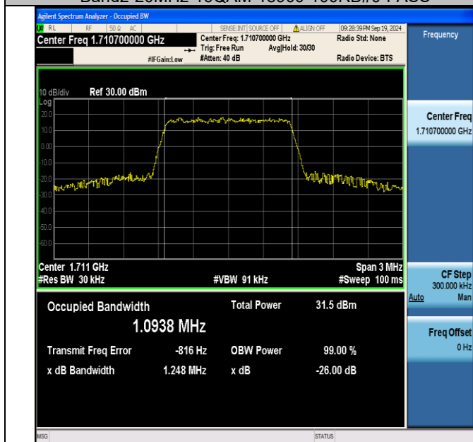
Band4-1.4MHz-QPSK-19957-6RB#0-PASS
