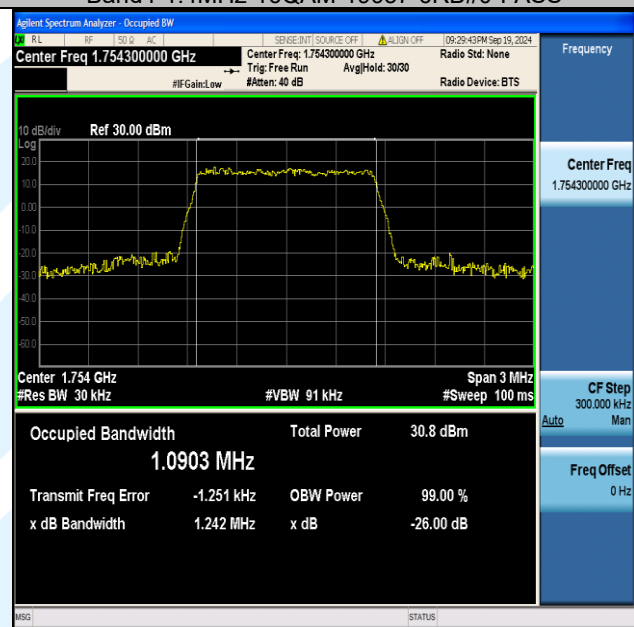
Band4-1.4MHz-16QAM-20393-6RB#0-PASS
