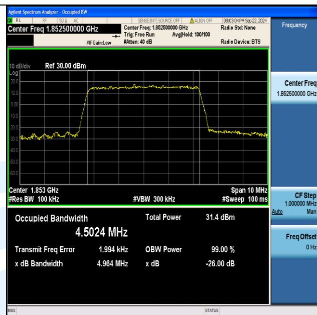
Band2-5MHz-16QAM-18625-25RB#0-PASS
