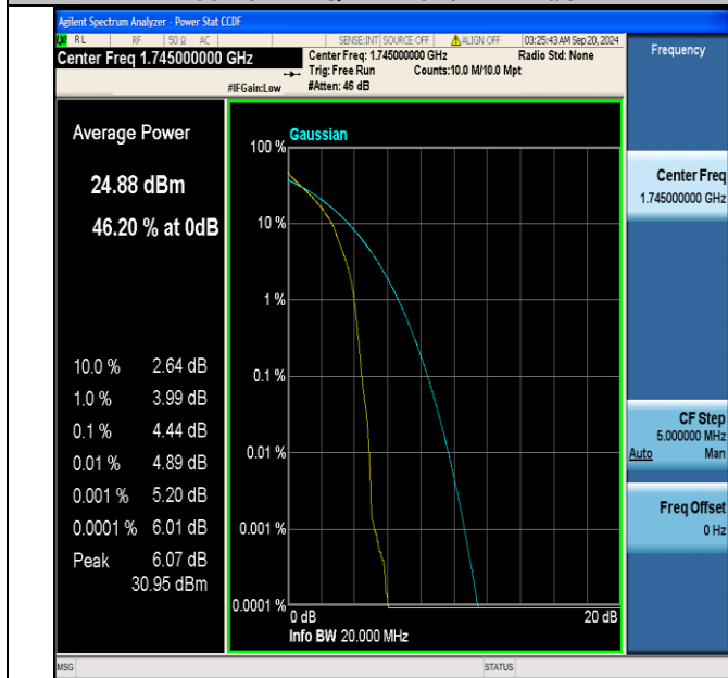
Band66-20MHz-QPSK-132322-1RB#0-PASS
