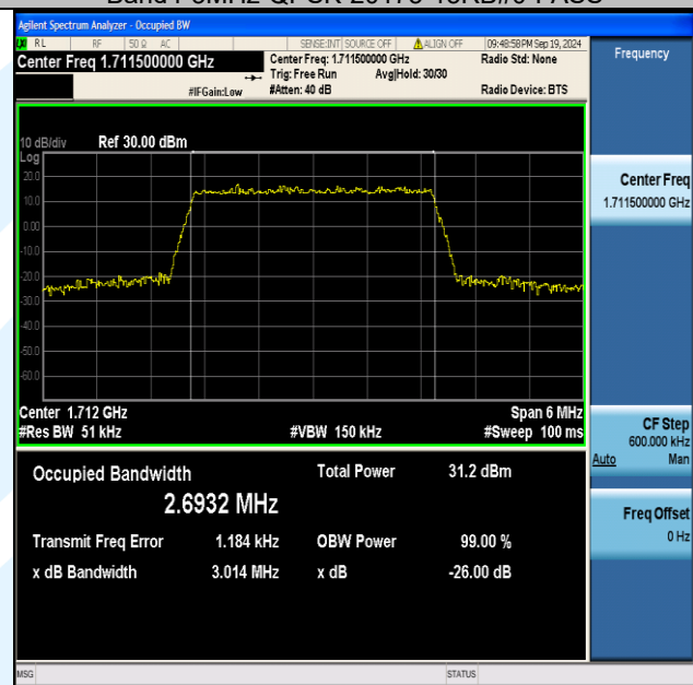
Band4-3MHz-16QAM-19965-15RB#0-PASS
