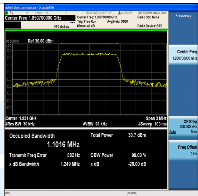
Band2-1.4MHz-16QAM-18607-6RB#0-PASS
