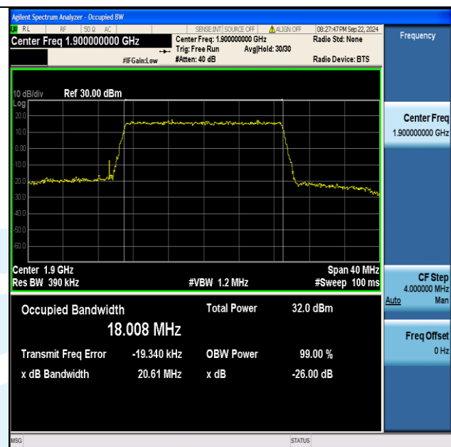
Band2-20MHz-16QAM-19100-100RB#0-PASS
