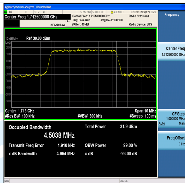
Band4-5MHz-16QAM-19975-25RB#0-PASS
