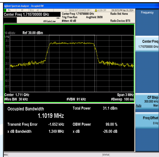
Band4-1.4MHz-16QAM-19957-6RB#0-PASS
