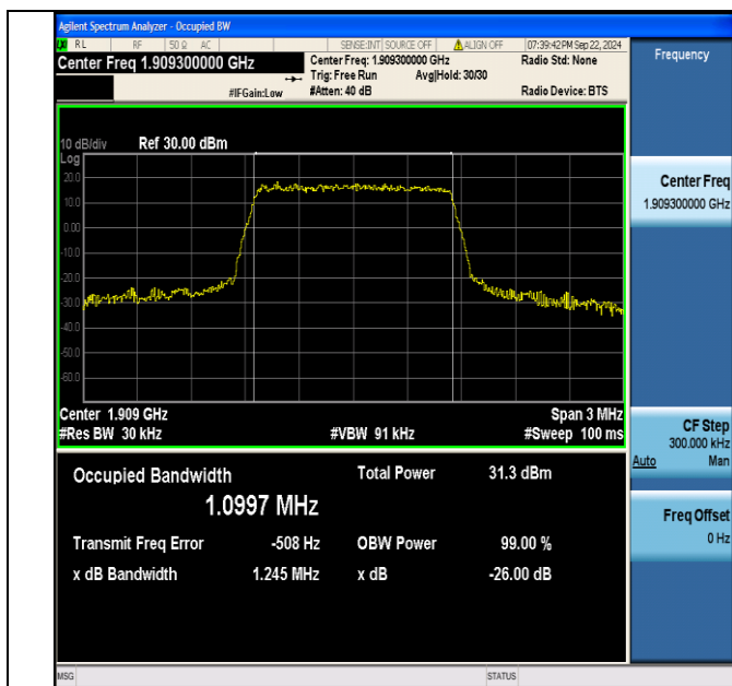
Band2-1.4MHz-QPSK-19193-6RB#0-PASS
