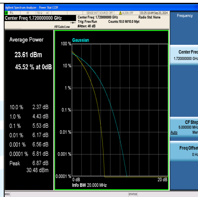
Band66-20MHz-QPSK-132072-100RB#0-PASS
