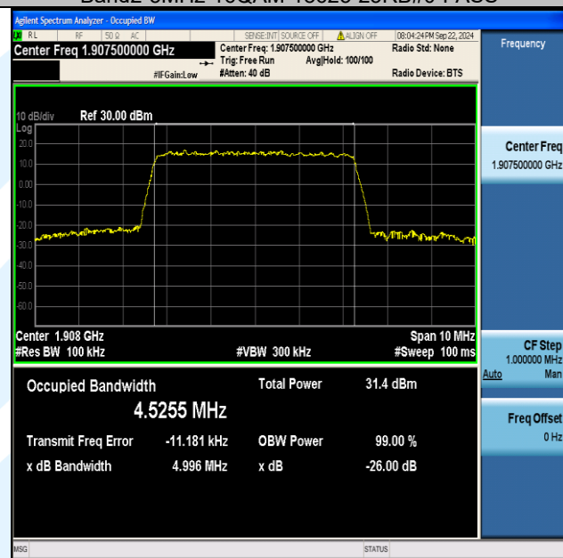
Band2-5MHz-16QAM-19175-25RB#0-PASS
