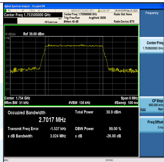
Band4-3MHz-16QAM-20385-15RB#0-PASS
