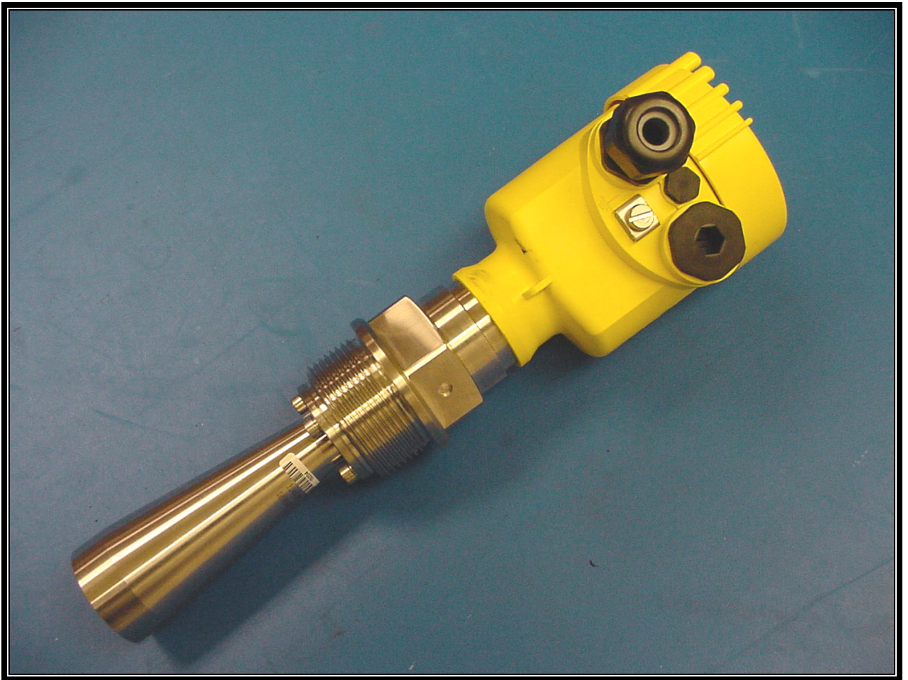
PHOTOGRAPH 15: EUT WITH 19.5 DBI HORN ANTENNA
