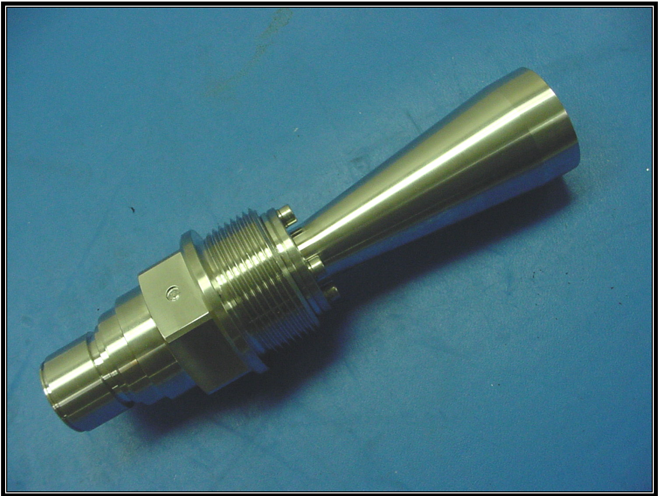
PHOTOGRAPH 16: 19.5 DBI HORN ANTENNA
