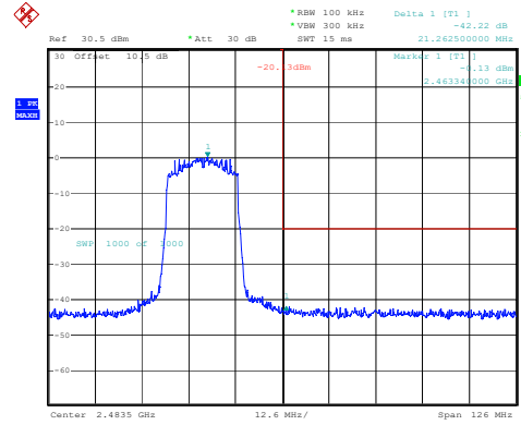
802.11ax20_2462MHz_RU_Full_Chain 2
