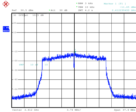
802.11ax20_2412MHz_RU_Full_Chain 1
