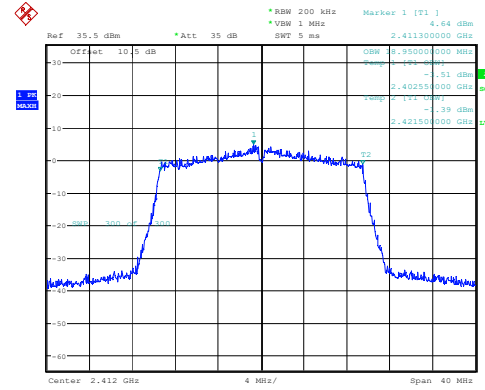
802.11ax20_2412MHz_RU_Full_Chain 2
