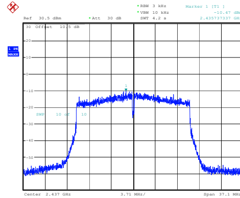
802.11ax20_2437MHz_RU_Full_Chain 1
