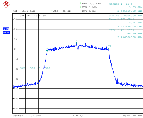
802.11ax20_2437MHz_RU_Full_Chain 2
