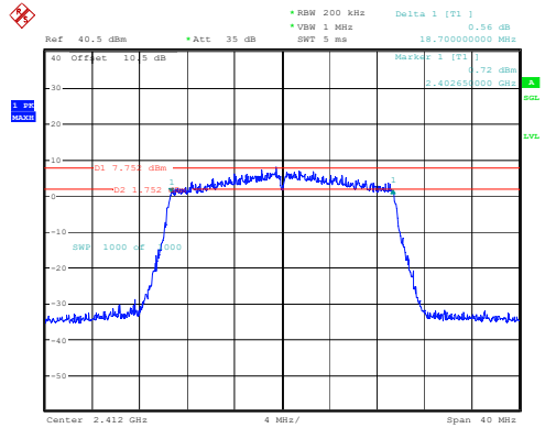
802.11ax20_2412MHz_RU_Full_Chain 1
