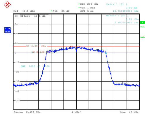
802.11ax20_2412MHz_RU_Full_Chain 2
