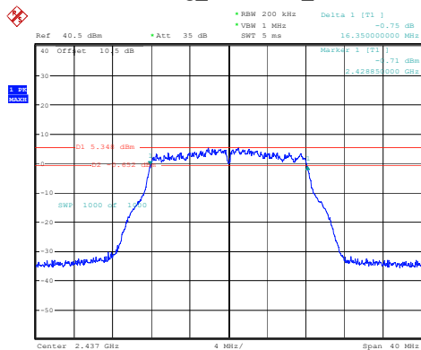
802.11g_2437MHz_Chain 2
