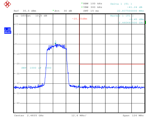
802.11ax20_2462MHz_RU_Full_Chain 1
