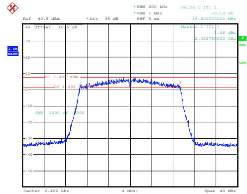
802.11ax20_2462MHz_RU_Full_Chain 2
