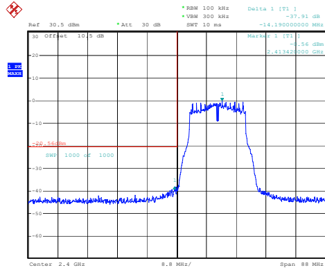
802.11g_2412MHz_Chain 2
