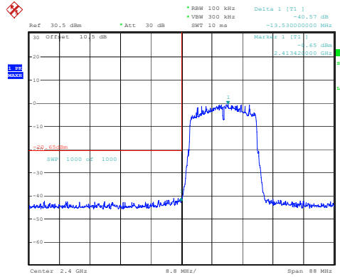
802.11ax20_2412MHz_RU_Full_Chain 1
