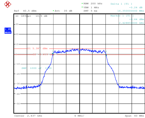
802.11g_2437MHz_Chain 1
