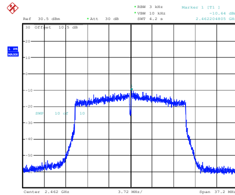
802.11ax20_2462MHz_RU_Full_Chain 2
