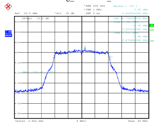
802.11g_2462MHz_Chain 2
