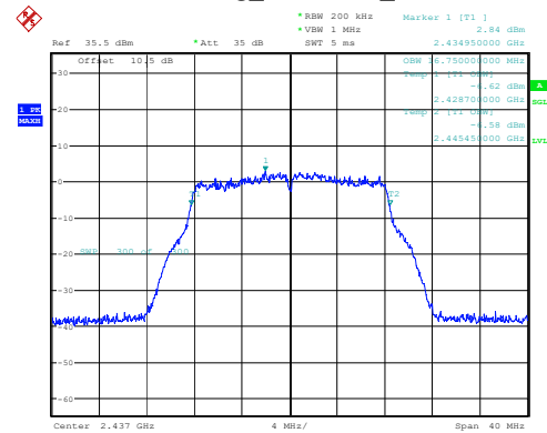
802.11g_2437MHz_Chain 1
