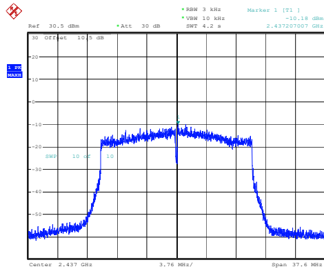
802.11ax20_2437MHz_RU_Full_Chain 2
