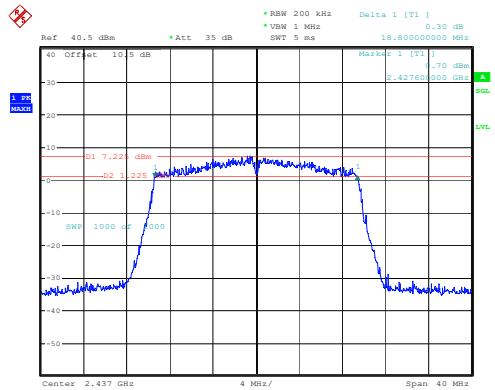
802.11ax20_2437MHz_RU_Full_Chain 2
