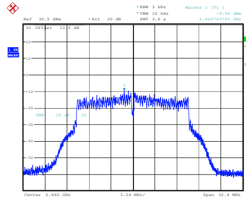
802.11g_2462MHz_Chain 2
