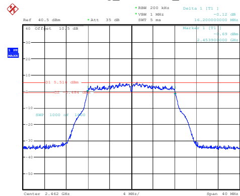
802.11g_2462MHz_Chain 2
