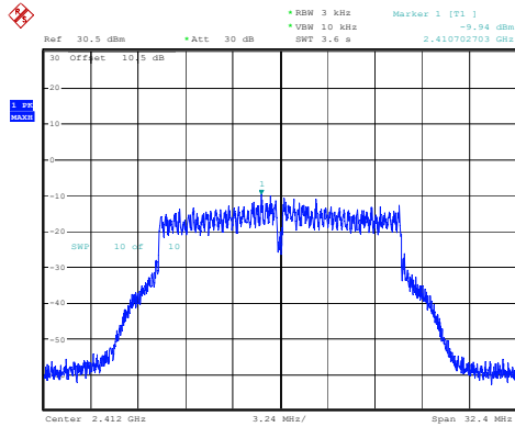
802.11g_2412MHz_Chain 1
