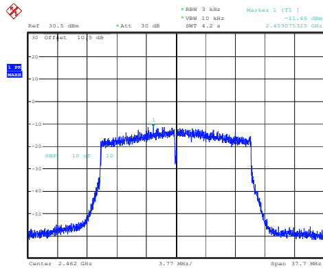
802.11ax20_2462MHz_RU_Full_Chain 1
