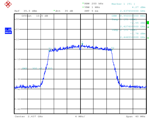
802.11ax20_2437MHz_RU_Full_Chain 1
