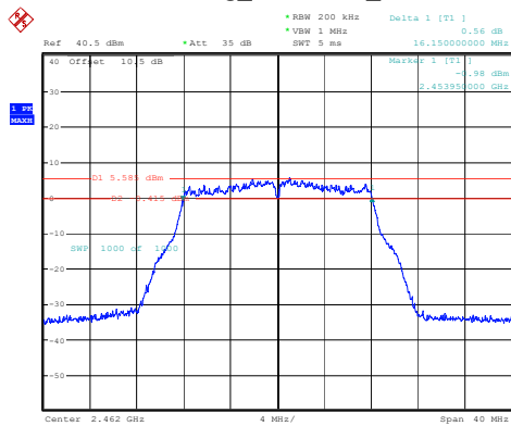
802.11g_2462MHz_Chain 1
