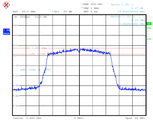
802.11ax20_2462MHz_RU_Full_Chain 1
