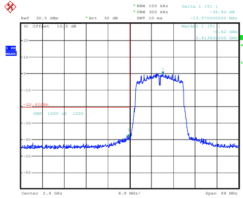
802.11ax20_2412MHz_RU_Full_Chain 2
