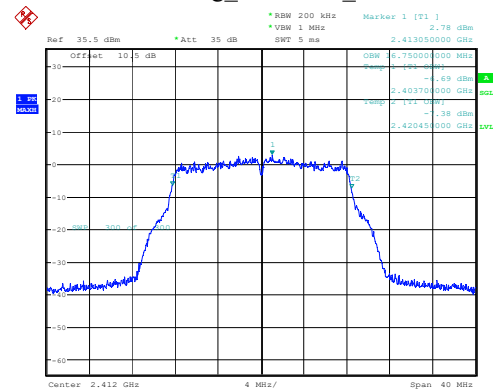
802.11g_2412MHz_Chain 2
