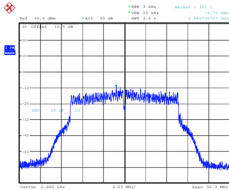
802.11g_2462MHz_Chain 1
