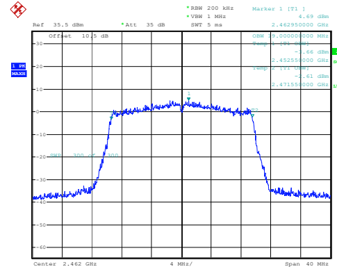
802.11ax20_2462MHz_RU_Full_Chain 2
