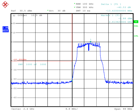
802.11g_2412MHz_Chain 1
