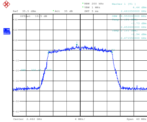
802.11ax20_2462MHz_RU_Full_Chain 1
