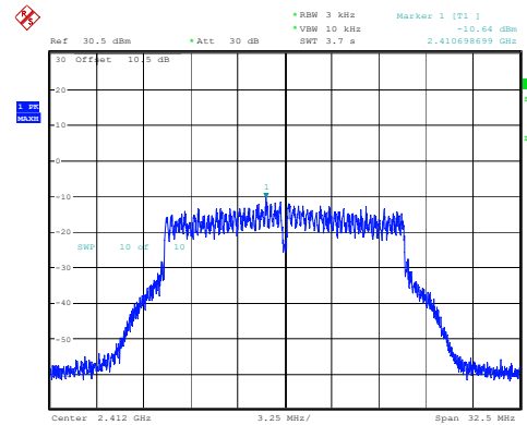
802.11g_2412MHz_Chain 2
