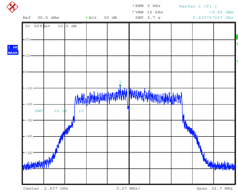
802.11g_2437MHz_Chain 1
