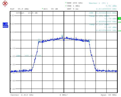
802.11ax20_2412MHz_RU_Full_Chain 1
