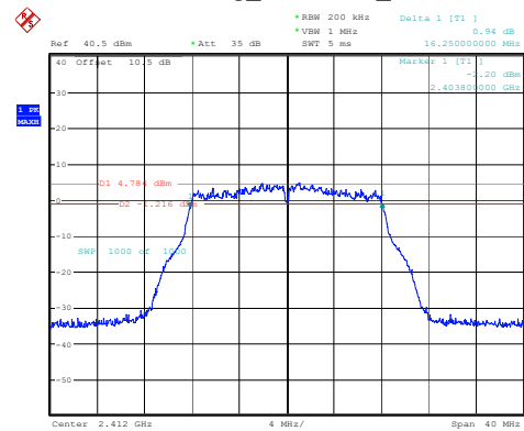
802.11g_2412MHz_Chain 2
