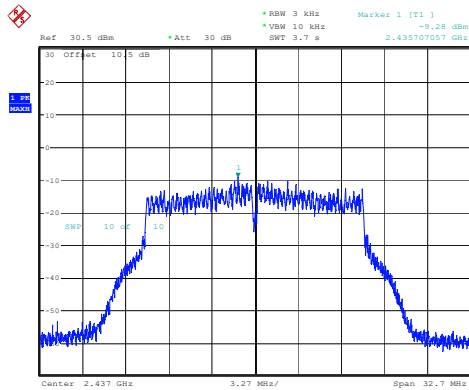
802.11g_2437MHz_Chain 2
