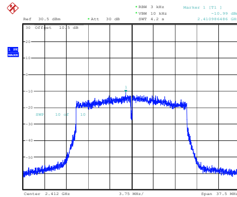
802.11ax20_2412MHz_RU_Full_Chain 2
