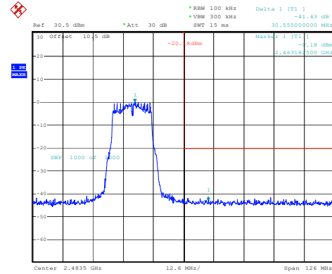
802.11g_2462MHz_Chain 2
