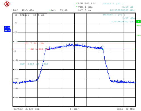
802.11ax20_2437MHz_RU_Full_Chain 1
