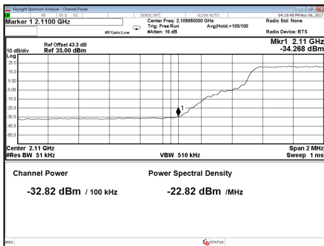
Figure 8.2-207: Conducted band edge emission at 2110 MHz, Port D, LTE, 10 MHz channel, 2 bottom carriers, QPSK (RBW = 1% of EBW)
