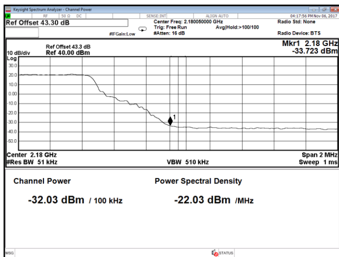
Figure 8.2-267: Conducted band edge emission at 2180 MHz, Port B, LTE, 10 MHz channel, 2 top carriers, QPSK (RBW = 1% of EBW)
