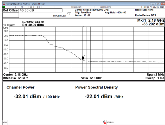
Figure 8.2-265: Conducted band edge emission at 2180 MHz, Port A, LTE, 10 MHz channel, 2 top carriers, QPSK (RBW = 1% of EBW)
