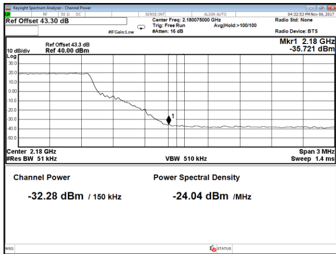
Figure 8.2-273: Conducted band edge emission at 2180 MHz, Port A, LTE, 15 MHz channel, 2 top carriers, QPSK (RBW = 1% of EBW)
