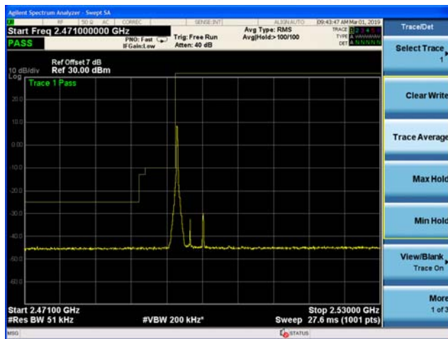
LTE Band 41 QPSK 5MHz CH-Low, 100%RB
