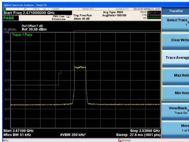
LTE Band 41 QPSK 10MHz CH-Low, 1 RB
