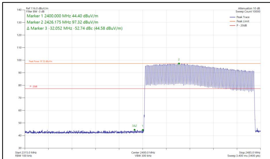
Figure 37 - Bluetooth DH5, SISO, Core 0 - Hopping Band Edge Frequency 2400 MHz
