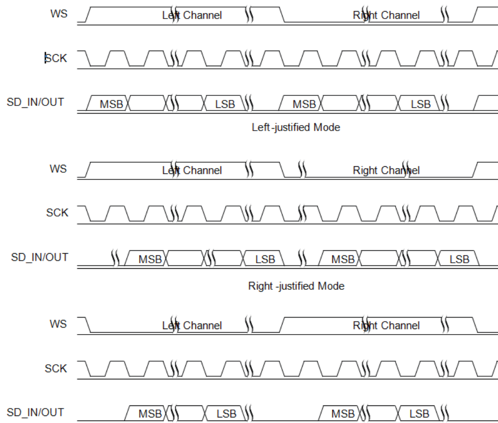
Figure 13: PCM Configuration
