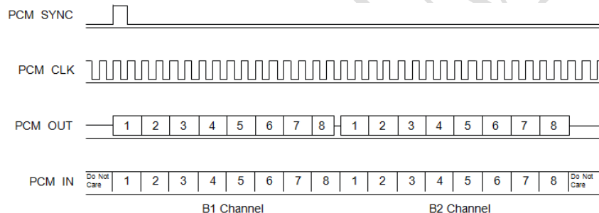
Figure 7: Multi-slot Operation
