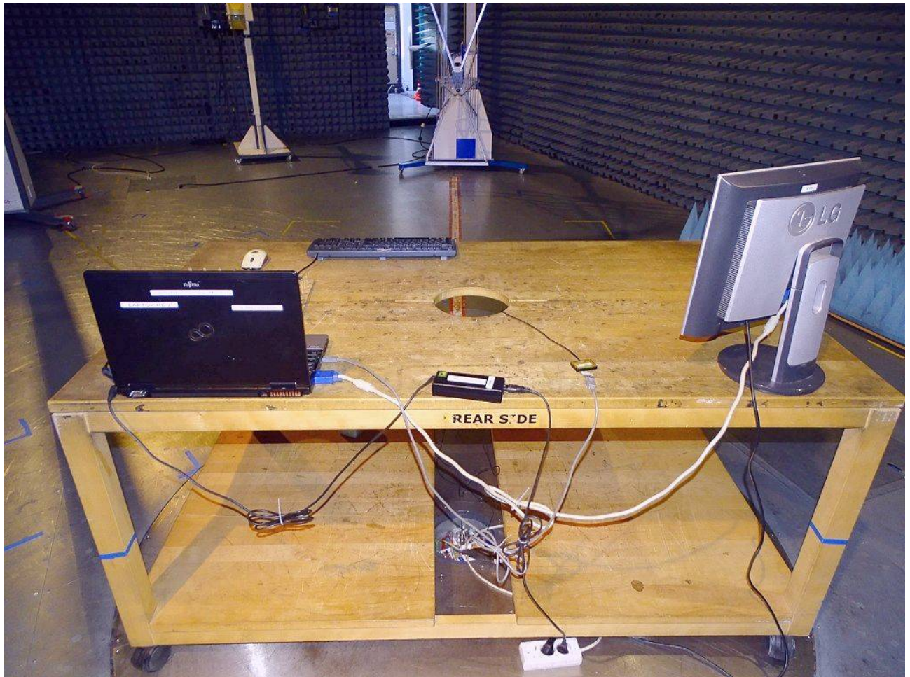
Photo 7: Test setup for radiated measurements (computer peripheral setup, EUT supplied by USB-cable from computer, unintentional radiator §15.109, ANSI C63.4) Frequency Range: 30 MHz – 1 GHz
