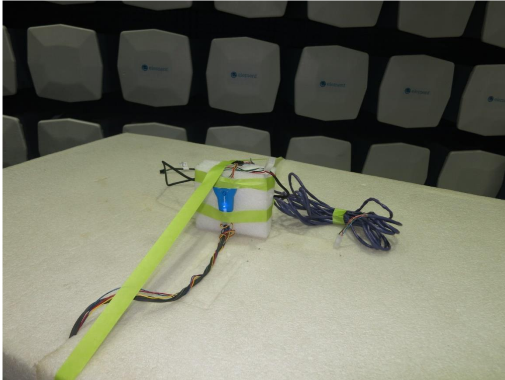
Radiated Spurious - BluKey+
