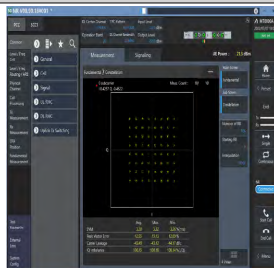
1-N26-824-849--15-20-M-8-CP-64QAM-Outer_Full-106@0-Ant1-see graph-PASS
