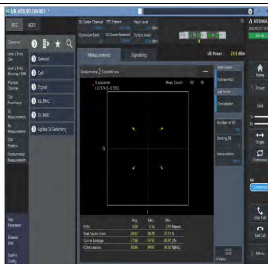
1-N26-824-849--15-20-M-2-DFT-QPSK-Out_Full-1 00@0-Ant1-see graph-PASS
