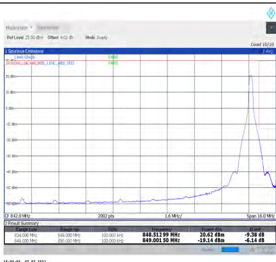
1-N26-824-849--15-15-H-2-DFT-PI2BPSK-Edge_1RB_Right-1@78-Ant1-seegraph-PASS-see graph
