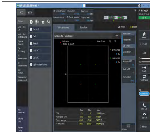
1-N26-824-849--15-20-M-1-DFT-PI2BPSK-Out_Full -100@0-Ant1-see graph-PASS
