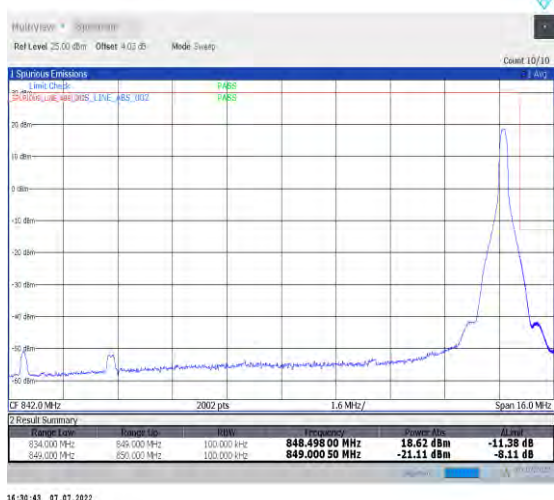
1-N26-824-849--15-15-H-5-CP-QPSK-Edge_1RB_Rig ht-1@78-Ant1-seegraph-PASS-see graph
