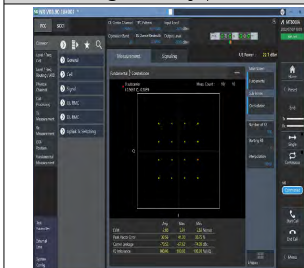
1-N26-824-849--15-20-M-3-DFT-16QAM-Out_Full-1 00@0-Ant1-see graph-PASS
