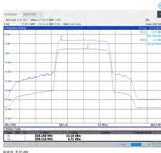
1-N26-824-849--15-20-M-2-CP-256QAM-Outer_Full-106@0-Ant1-9.47-100%-0.00-9.47-PASS-≤13
