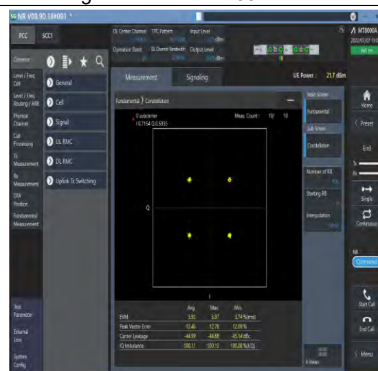
1-N26-824-849--15-20-M-6-CP-QPSK-Outer_Full-106@0-Ant1-see graph-PASS
