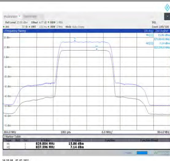
1-N26-824-849--15-20-L-1-DFT-256QAM-Outer_Full-100@0-Ant1-8.72-100%-0.00-8.72-PASS-≤13
