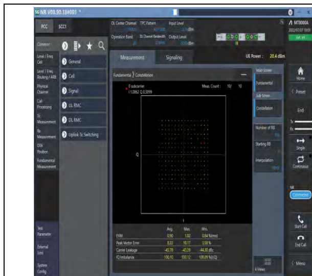
1-N26-824-849--15-20-M-5-DFT-256QAM-Outer_Full-100@0-Ant1-see graph-PASS
