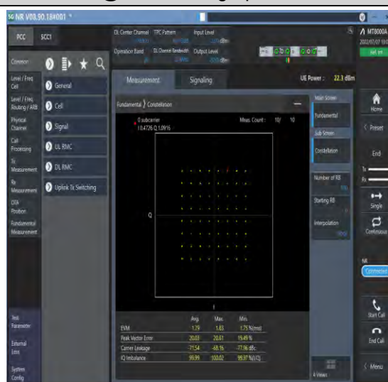
1-N26-824-849--15-20-M-4-DFT-64QAM-Out_Full -100@0-Ant1-see graph-PASS
