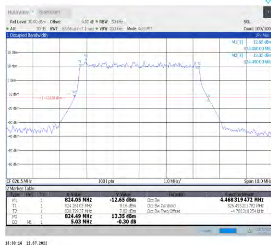
1-N26-824-849--15-5-L-2-DFT-PI2BPSK-Outter_Full-25@0-Ant1-4.465-5.010-≤5-PASS
