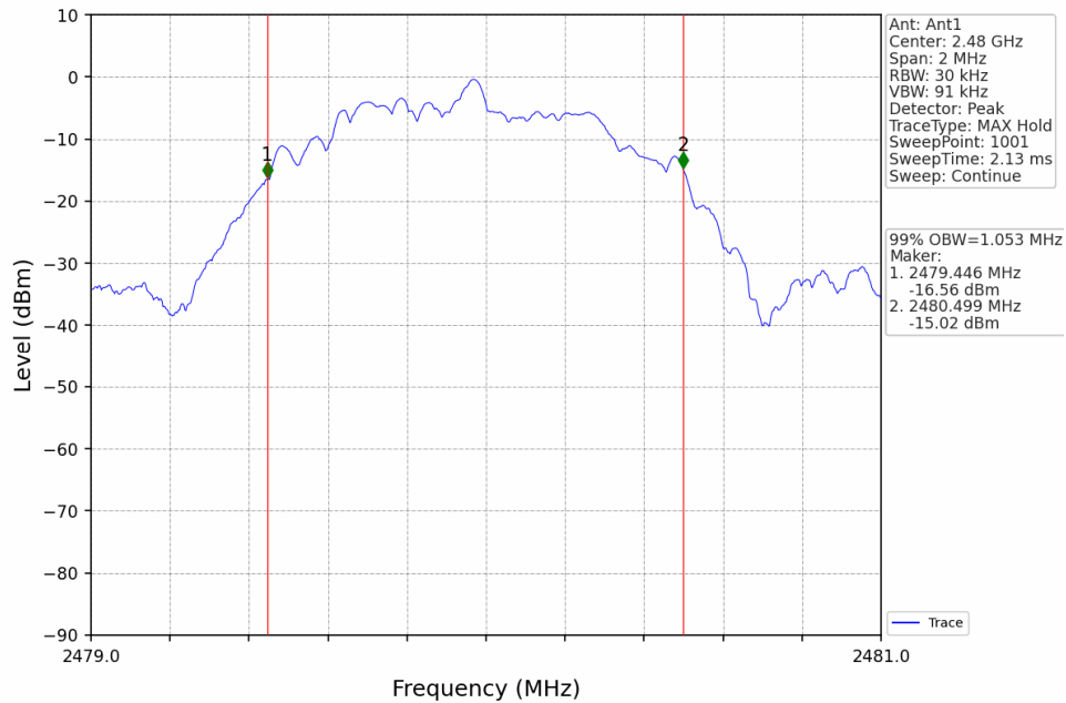
1M_HCH_2480MHz_Ant1_NTNV
