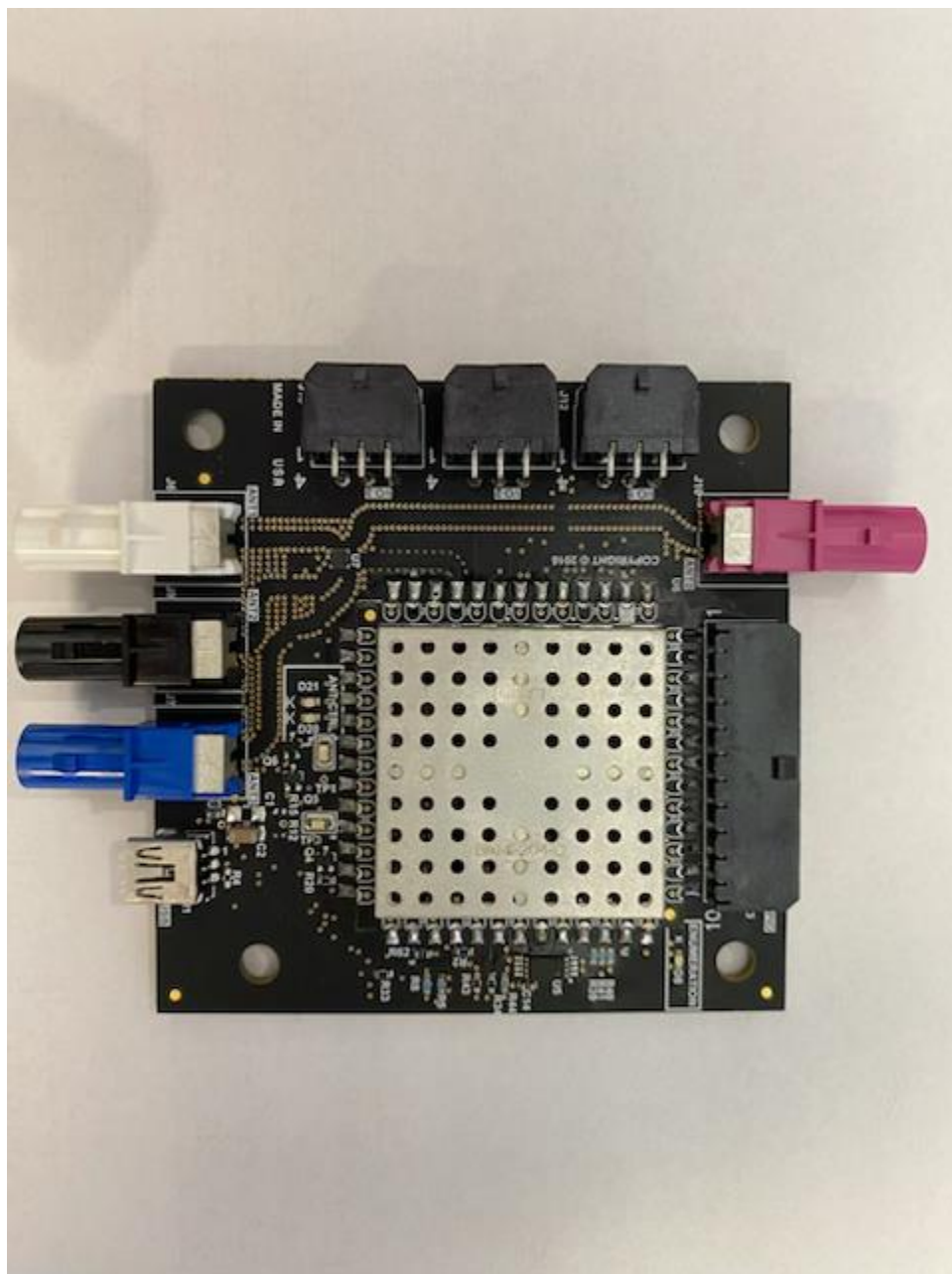
Figure 1: Top View
