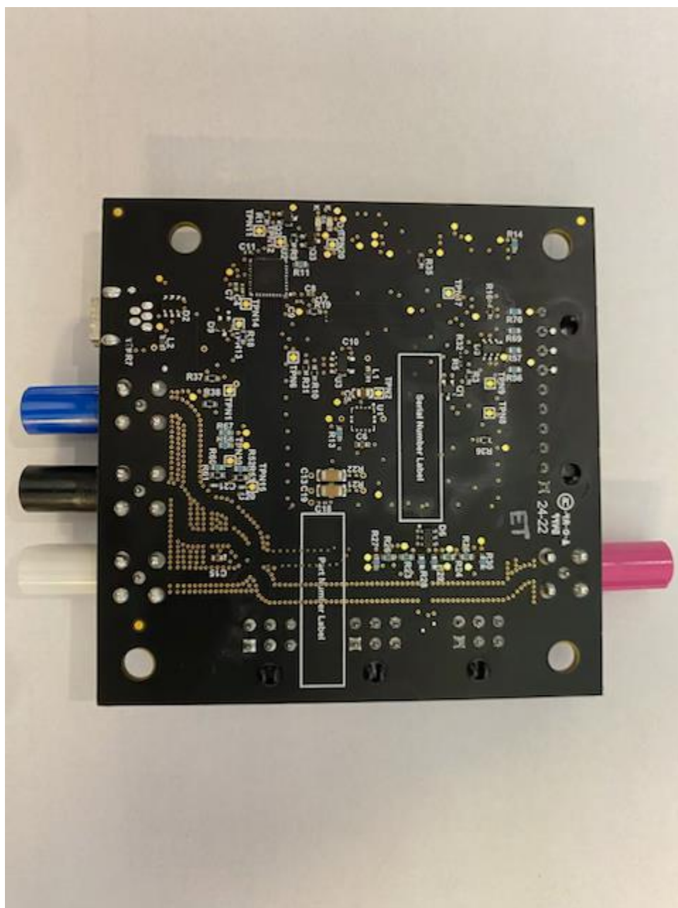
Figure 3: Bottom View
