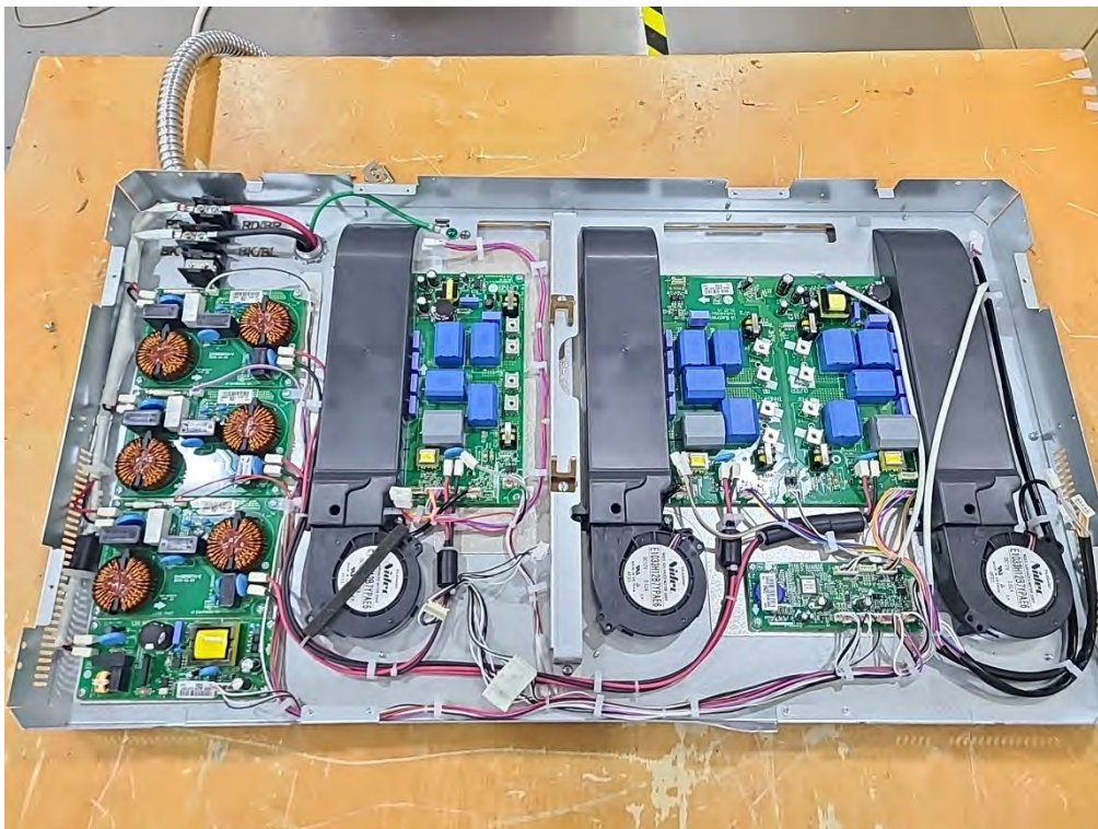
<Bottom plate>
