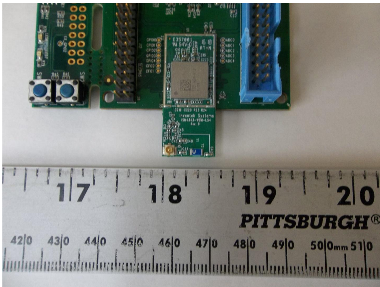
Figure 2. Close Up of Module Board on Test PCB
