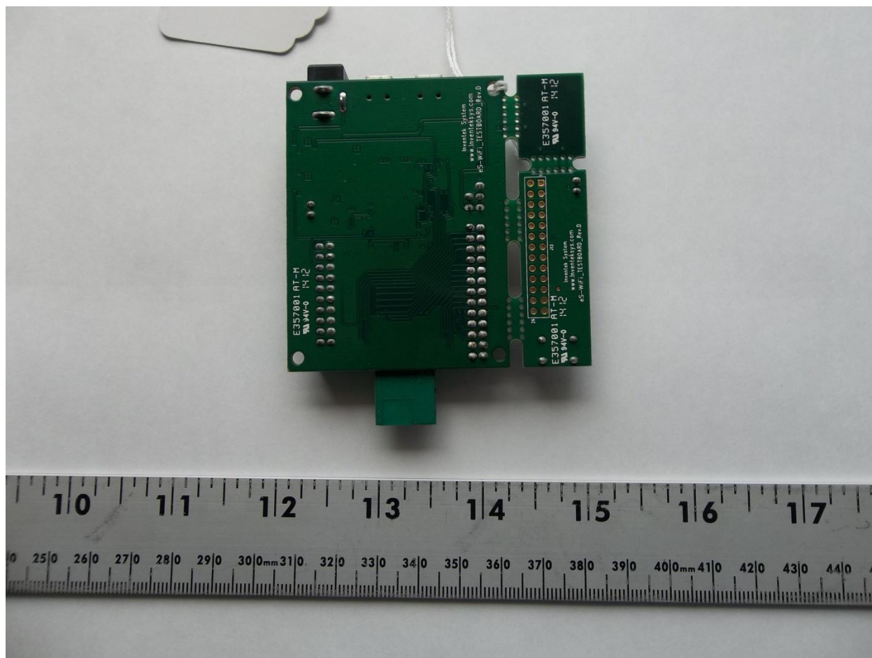
Figure 2. Back of PCB with Module
