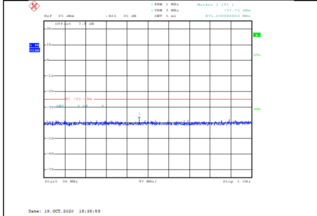
Band38-20MHz-16QAM-38150-1RB#0-Range1:30~1000MHz--37.75-PASS
