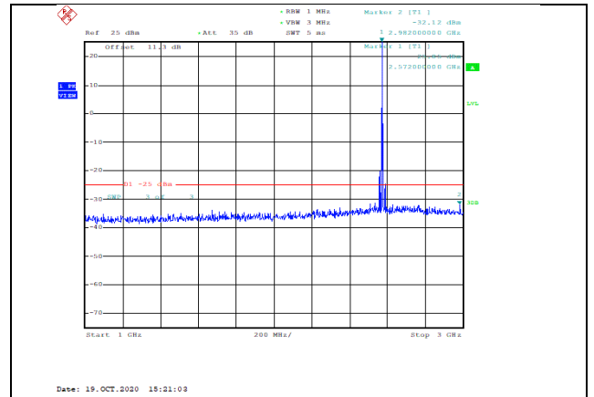
Band38-5MHz-16QAM-37775-1RB#0-Range2:1000~3000MHz--32.12-PASS
