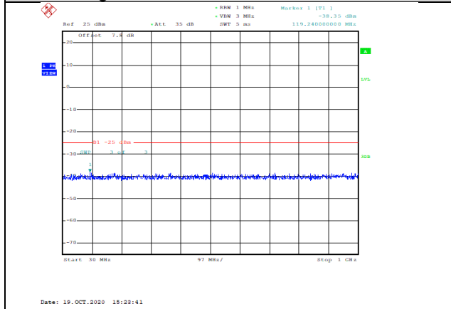
Band38-5MHz-16QAM-38225-1RB#0-Range1:30~1000MHz--38.35-PASS
