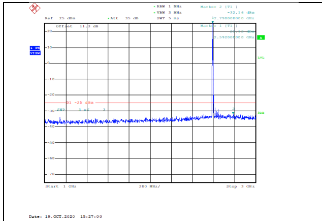
Band38-10MHz-16QAM-38000-1RB#0-Range2:1000~3000MHz--32.16-PASS
