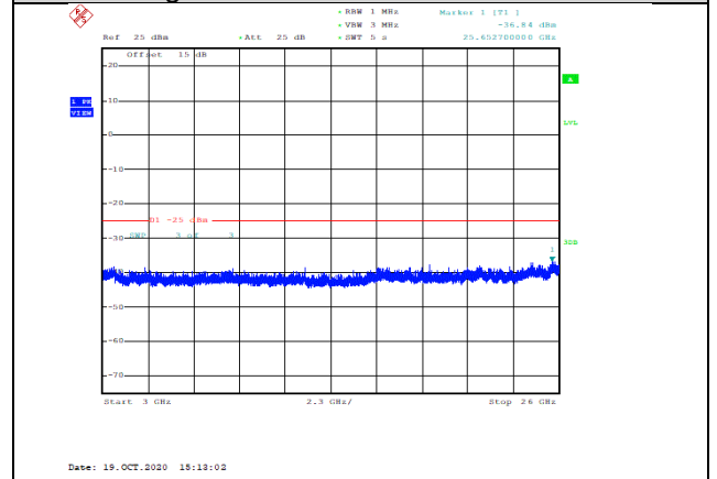
Band7-15MHz-QPSK-21100-1RB#0-Range3:3000~26000MHz--36.84-PASS
