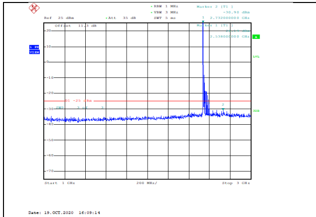
Band41-20MHz-QPSK-40140-1RB#0- Range2:1000~3000MHz--30.9-PASS
