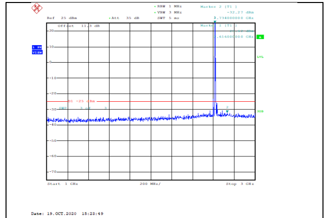
Band38-5MHz-16QAM-38225-1RB#0-Range2:1000~3000MHz--32.27-PASS
