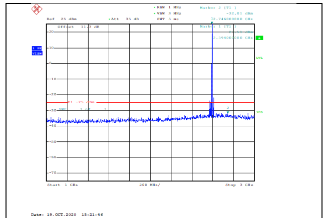
Band38-5MHz-QPSK-38000-1RB#0-Range2:1000~3000MHz--32.01-PASS
