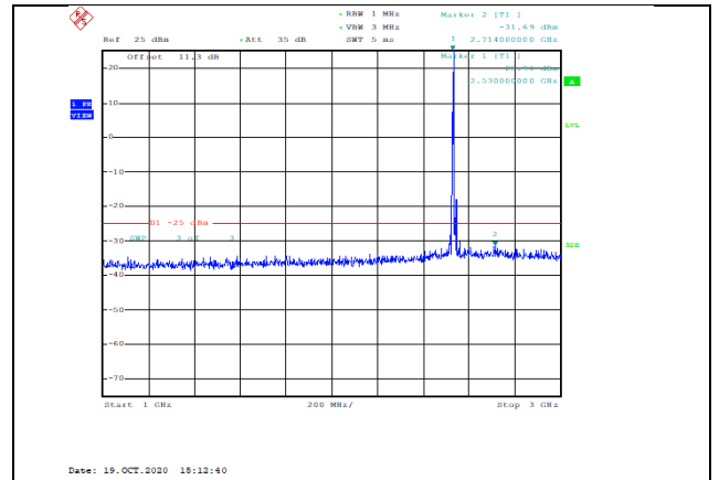
Band7-15MHz-QPSK-21100-1RB#0-Range2:1000~3000MHz--31.69-PASS
