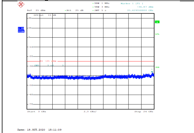
Band7-15MHz-QPSK-20825-1RB#0-Range3:3000~26000MHz--36.87-PASS
