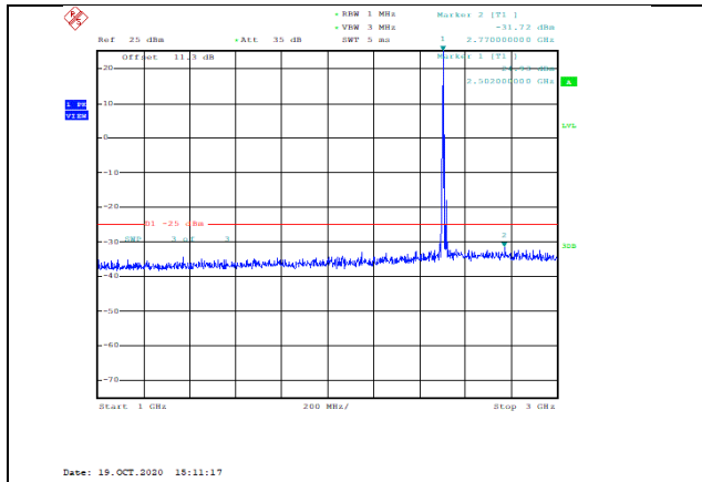
Band7-15MHz-QPSK-20825-1RB#0-Range2:1000~3000MHz--31.72-PASS
