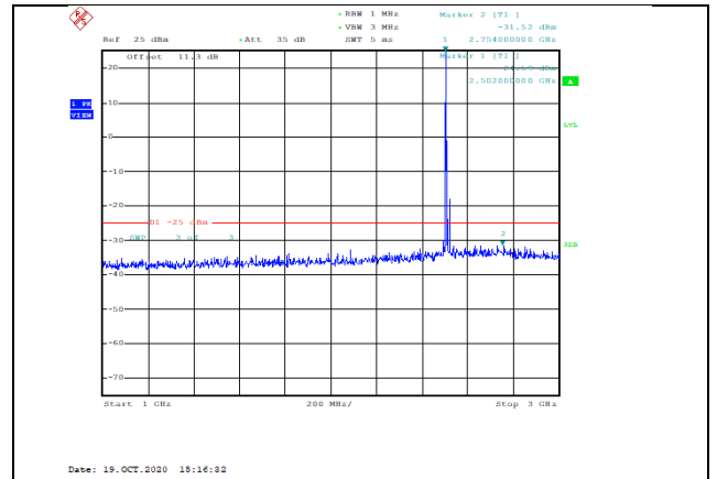
Band7-20MHz-16QAM-20850-1RB#0-Range2:1000~3000MHz--31.52-PASS
