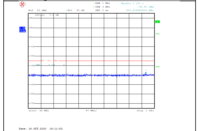
Band41-20MHz-QPSK-41140-1RB#0- Range1:30~1000MHz--38.45-PASS
