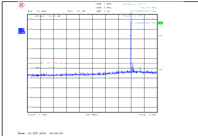
Band38-5MHz-16QAM-38000-1RB#0-Range2:1000~3000MHz--32.18-PASS
