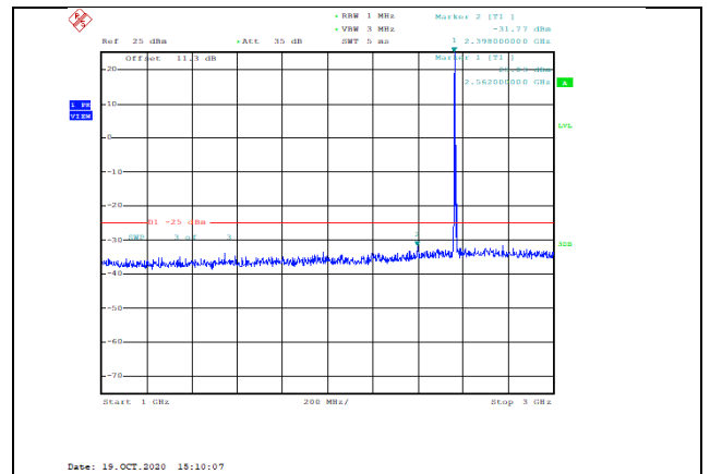
Band7-10MHz-16QAM-21400-1RB#0-Range2:1000~3000MHz--31.77-PASS
