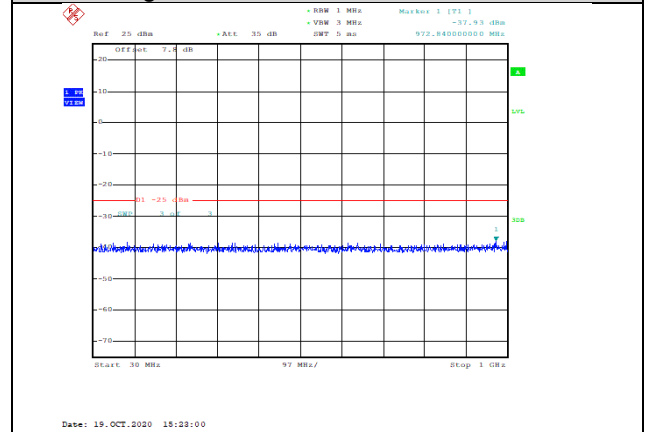
Band38-5MHz-QPSK-38225-1RB#0-Range1:30~1000MHz--37.93-PASS
