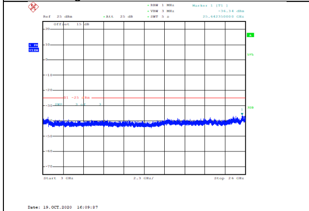
Band41-20MHz-QPSK-40140-1RB#0- Range3:3000~26000MHz--36.34-PASS
