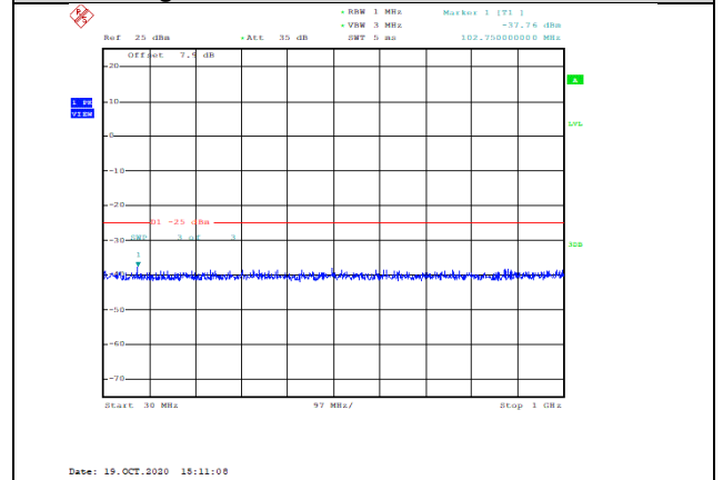
Band7-15MHz-QPSK-20825-1RB#0-Range1:30~1000MHz--37.76-PASS
