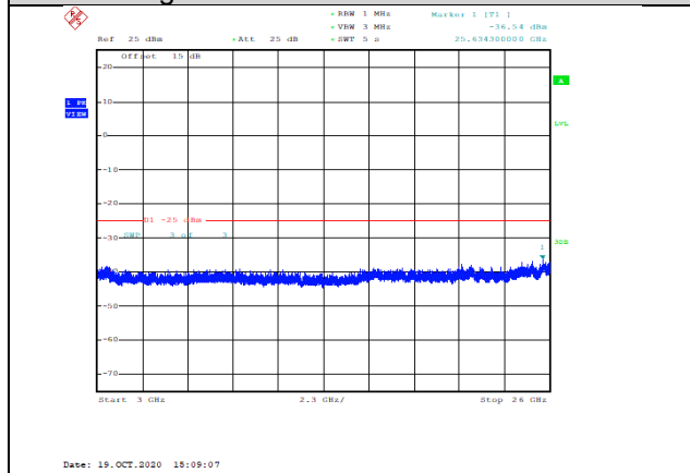
Band7-10MHz-16QAM-21100-1RB#0-Range3:3000~26000MHz--36.54-PASS
