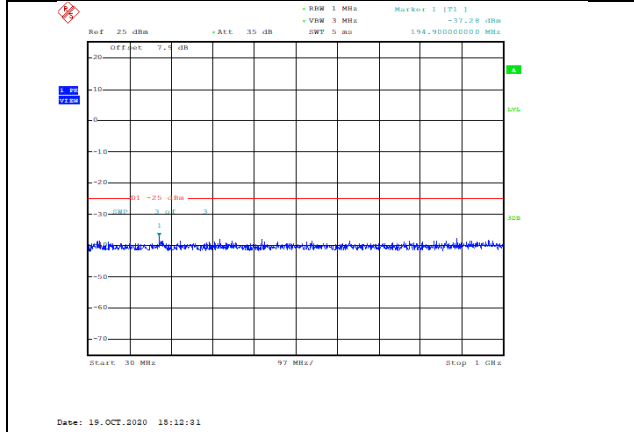
Band7-15MHz-QPSK-21100-1RB#0-Range1:30~1000MHz--37.28-PASS
