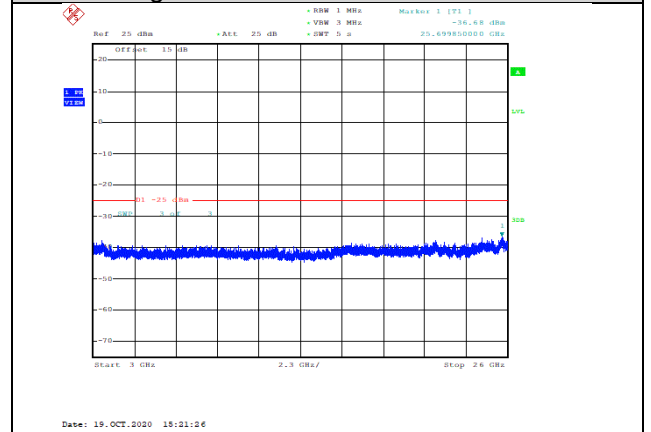
Band38-5MHz-16QAM-37775-1RB#0-Range3:3000~26000MHz--36.68-PASS
