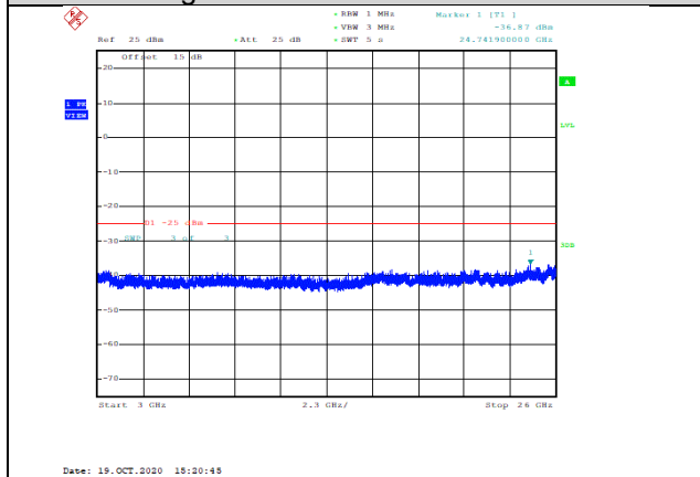
Band38-5MHz-QPSK-37775-1RB#0-Range3:3000~26000MHz--36.87-PASS
