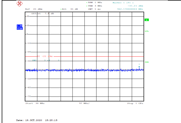
Band38-10MHz-16QAM-38200-1RB#0-Range1:30~1000MHz--37.25-PASS
