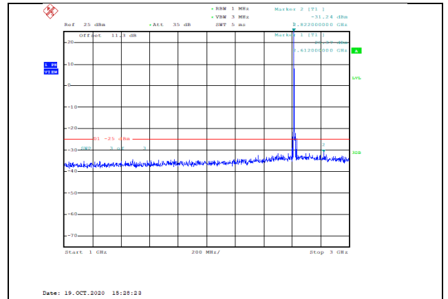
Band38-10MHz-16QAM-38200-1RB#0-Range2:1000~3000MHz--31.24-PASS
