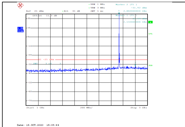
Band7-10MHz-16QAM-21100-1RB#0-Range2:1000~3000MHz--31.92-PASS
