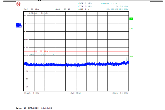
Band7-10MHz-16QAM-21400-1RB#0-Range3:3000~26000MHz--36.96-PASS
