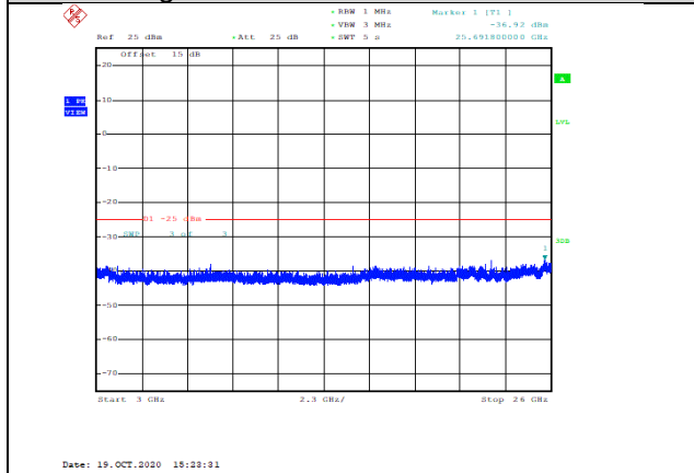
Band38-5MHz-QPSK-38225-1RB#0-Range3:3000~26000MHz--36.92-PASS
