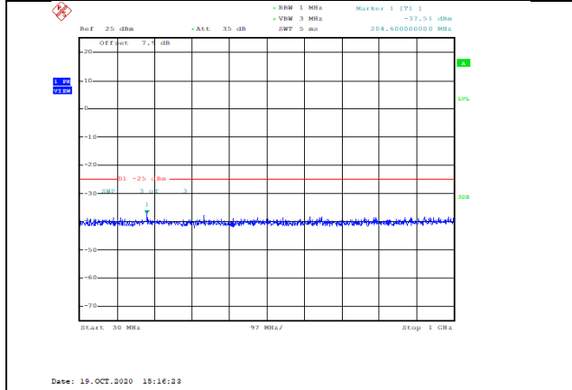
Band7-20MHz-16QAM-20850-1RB#0-Range1:30~1000MHz--37.51-PASS
