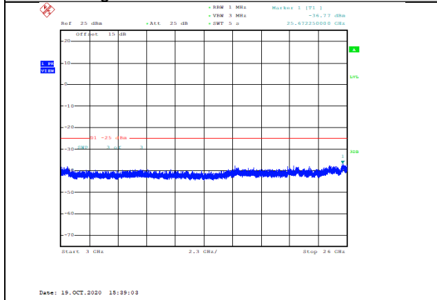
Band38-20MHz-16QAM-38000-1RB#0-Range3:3000~26000MHz--36.77-PASS
