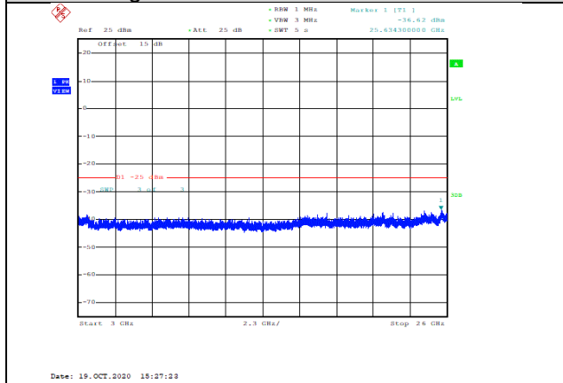
Band38-10MHz-16QAM-38000-1RB#0-Range3:3000~26000MHz--36.62-PASS
