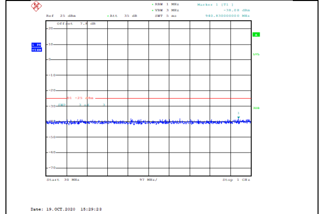
Band38-15MHz-QPSK-37825-1RB#0-Range1:30~1000MHz--38.08-PASS
