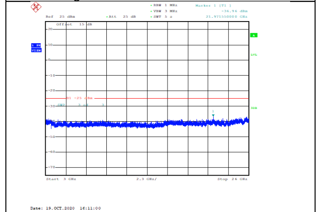
Band41-20MHz-QPSK-40590-1RB#0- Range3:3000~26000MHz--36.96-PASS
