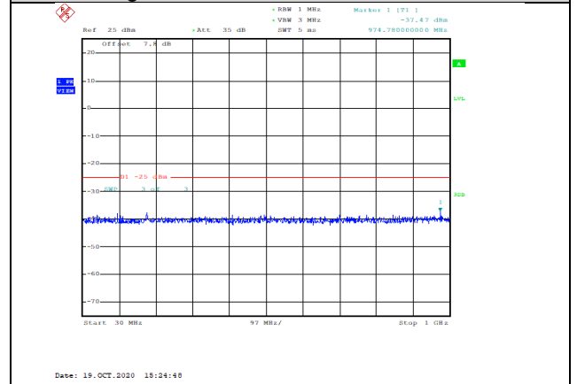
Band38-10MHz-QPSK-37800-1RB#0-Range1:30~1000MHz--37.47-PASS
