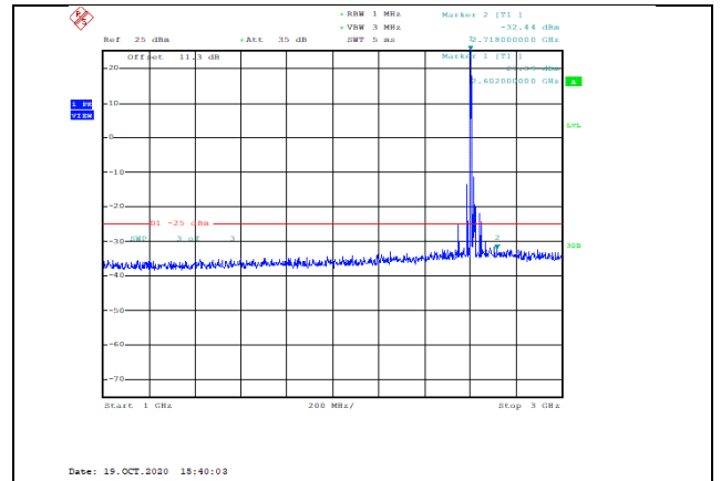
Band38-20MHz-16QAM-38150-1RB#0-Range2:1000~3000MHz--32.44-PASS
