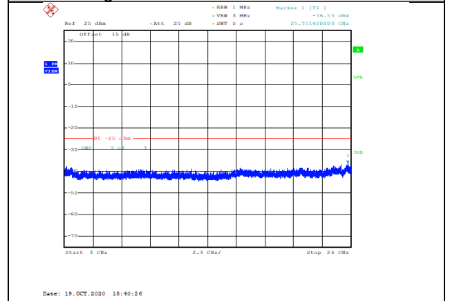
Band38-20MHz-16QAM-38150-1RB#0-Range3:3000~26000MHz--36.53-PASS
