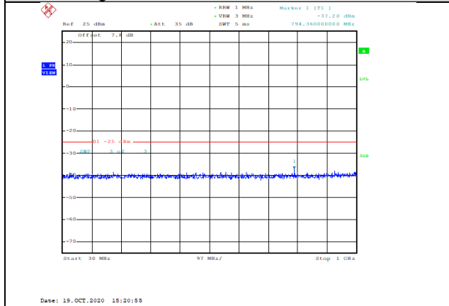
Band38-5MHz-16QAM-37775-1RB#0-Range1:30~1000MHz--37.2-PASS
