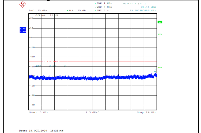
Band38-10MHz-16QAM-38200-1RB#0-Range3:3000~26000MHz--36.45-PASS
