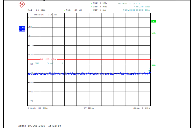
Band38-5MHz-16QAM-38000-1RB#0-Range1:30~1000MHz--38.3-PASS
