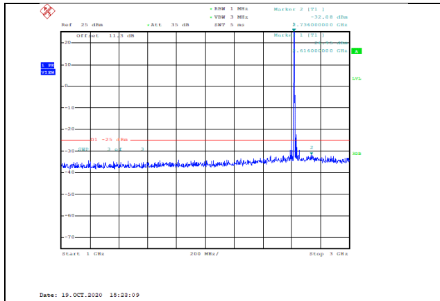
Band38-5MHz-QPSK-38225-1RB#0-Range2:1000~3000MHz--32.08-PASS
