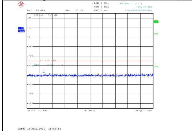
Band7-10MHz-16QAM-21400-1RB#0-Range1:30~1000MHz--38.13-PASS
