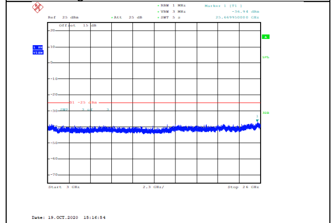
Band7-20MHz-16QAM-20850-1RB#0-Range3:3000~26000MHz--36.94-PASS
