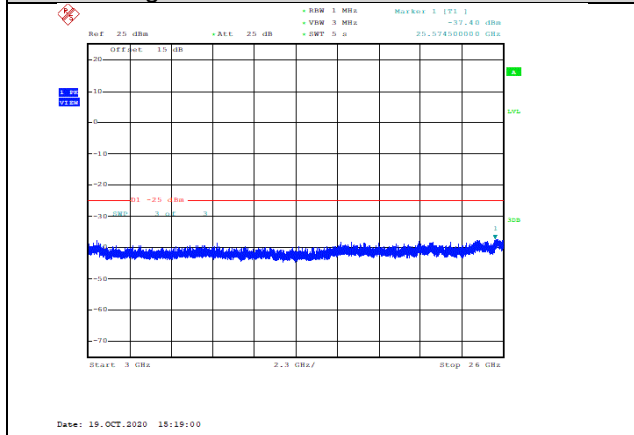
Band7-20MHz-QPSK-21350-1RB#0-Range3:3000~26000MHz--37.4-PASS
