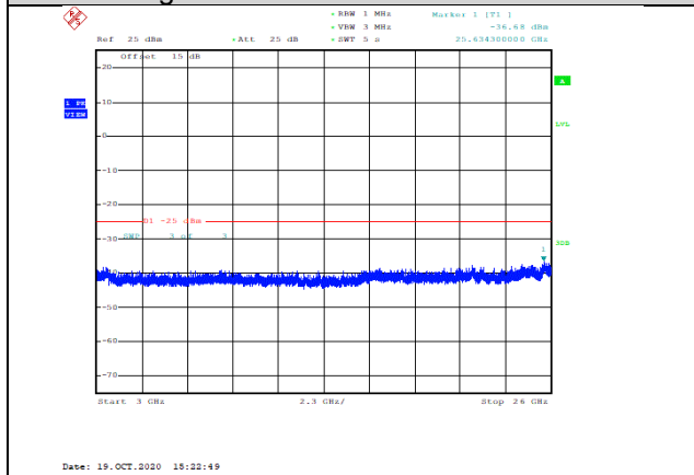
Band38-5MHz-16QAM-38000-1RB#0-Range3:3000~26000MHz--36.68-PASS
