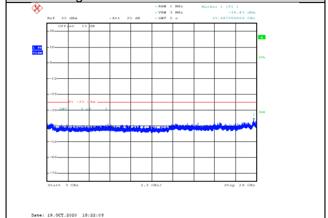
Band38-5MHz-QPSK-38000-1RB#0-Range3:3000~26000MHz--36.45-PASS
