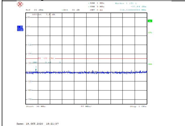
Band38-5MHz-QPSK-38000-1RB#0-Range1:30~1000MHz--37.84-PASS
