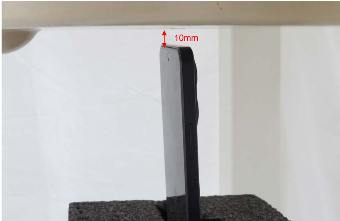
Picture 11: Top Edge, the distance from handset to the bottom of the Phantom is 10mm
