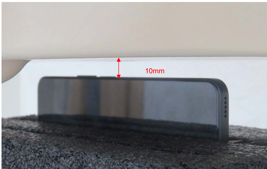
Picture 10: Right Edge, the distance from handset to the bottom of the Phantom is 10mm
