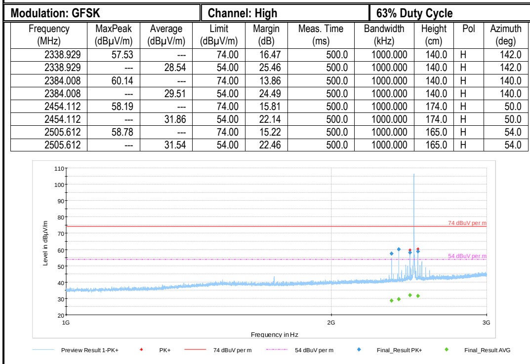
Plot # 10 Radiated Emissions: 1-3 GHz
