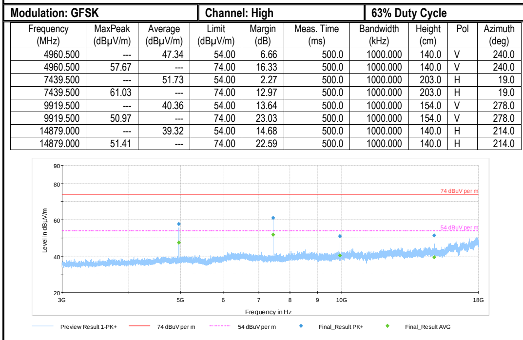
Plot # 11 Radiated Emissions: 3-18 GHz
