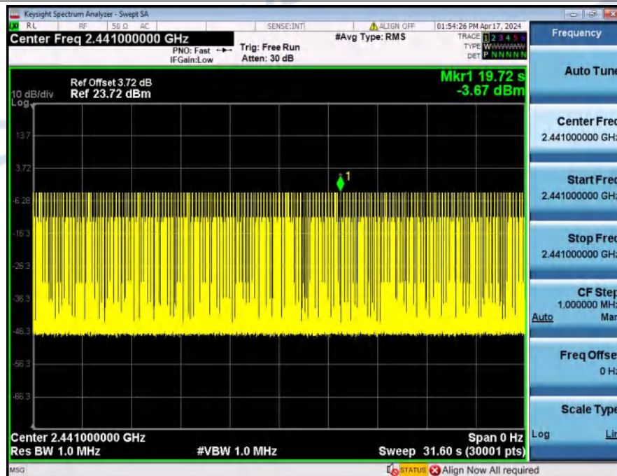
Dwell_Time_(Hopping)_NVNT_ANT1_1-DH1_2441_Accumulated
