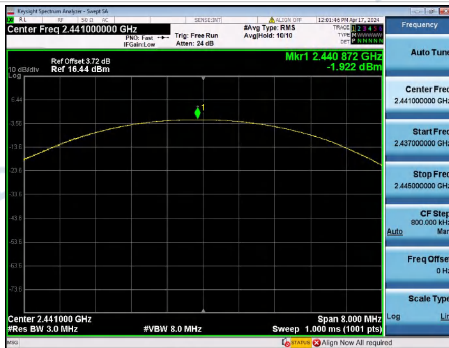
Peak_Output_Power_NVNT_ANT1_2-DH5_2441
