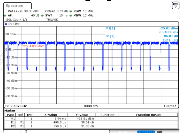
802.11n HT40_Ant1_2437MHz
