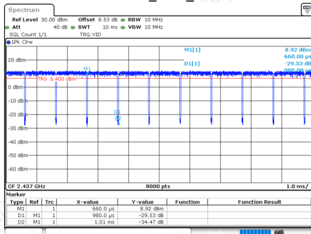
802.11n HT20_Ant1_2437MHz
