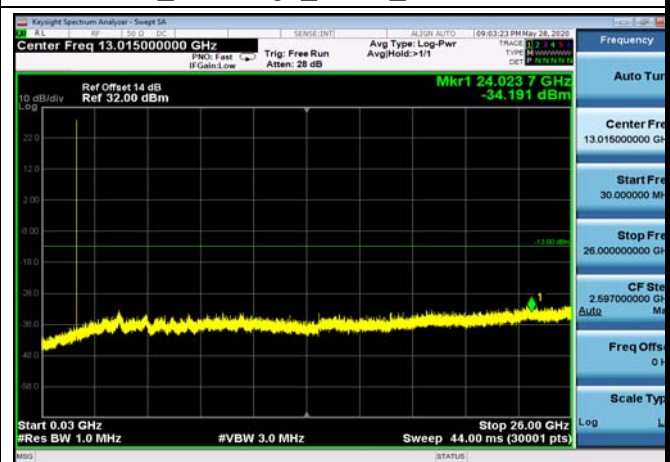
FDD66_MidRange_5MHz_30MHz~26GHz
