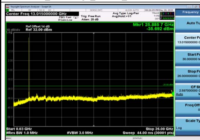
FDD07_LowRange_20MHz_30MHz~26GHz
