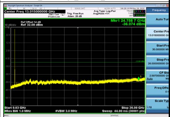
FDD26_MidRange_3MHz_30MHz~26GHz
