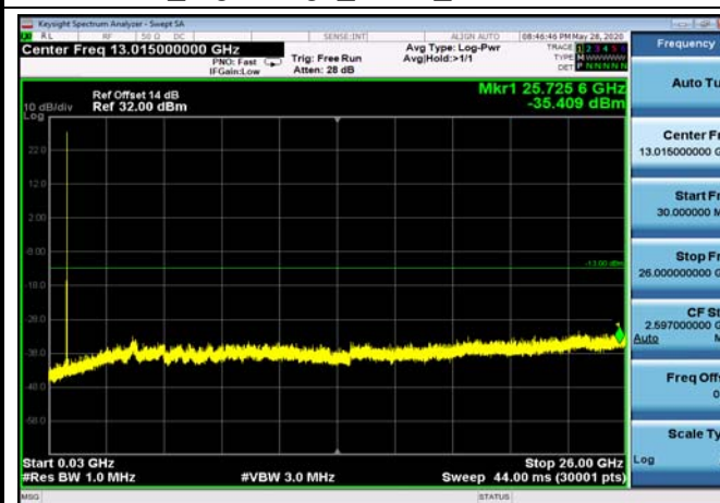
FDD26_LowRange_10MHz_30MHz~26GHz
