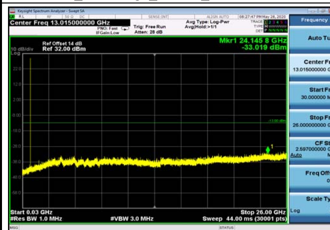
FDD26_LowRange_10MHz_30MHz~26GHz
