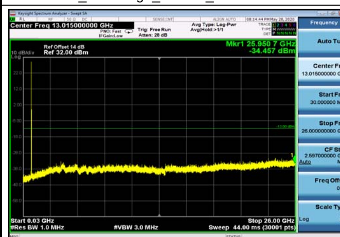
FDD26_MidRange_15MHz_30MHz~26GHz
