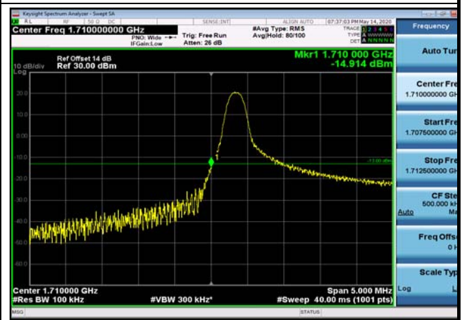
LowRange_FDD04_5MHz_1712.5_OneRB _low_Q16
