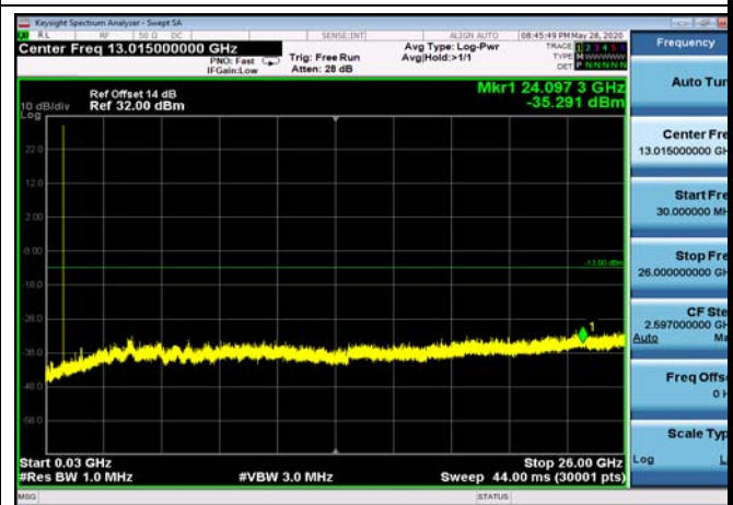
FDD26_MidRange_10MHz_30MHz~26GHz
