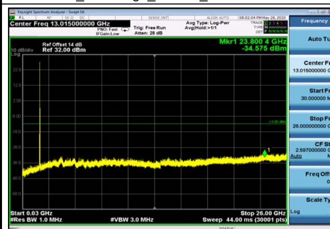
FDD66_MidRange_20MHz_30MHz~26GHz
