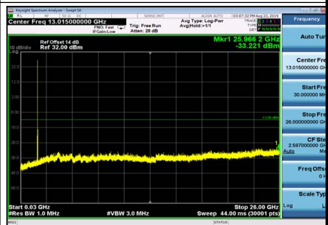
FDD66_MidRange_3MHz_30MHz~26GHz
