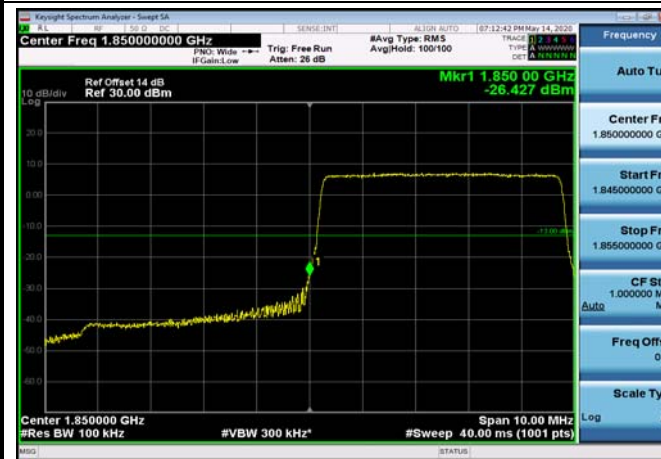
LowRange_FDD02_10MHz_1855_OneRB _low_QPSK
