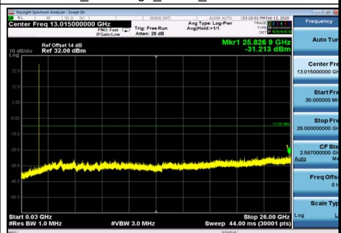
FDD66_MidRange_5MHz_30MHz~26GHz
