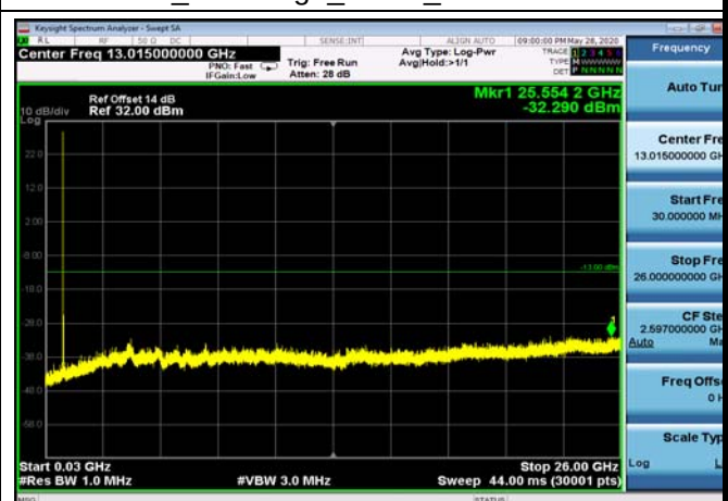
FDD26_MidRange_3MHz_30MHz~26GHz
