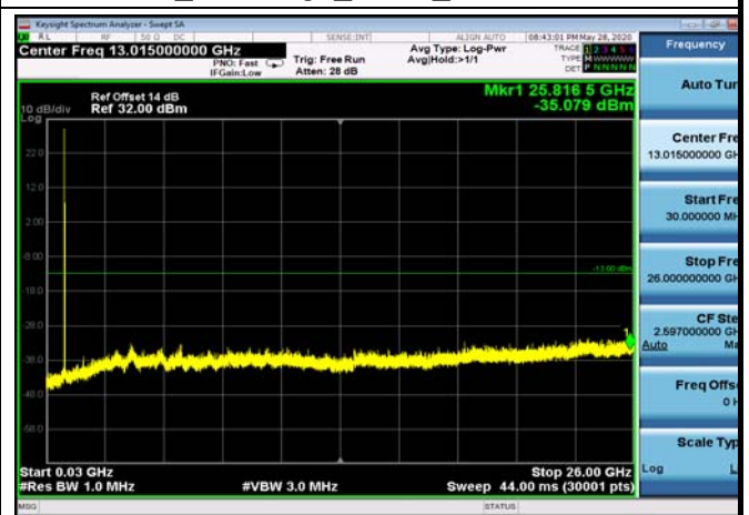
FDD07_HighRange_15MHz_30MHz~26GHz
