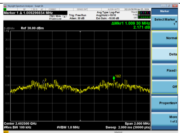
2DH5 | 1.009 MHz
