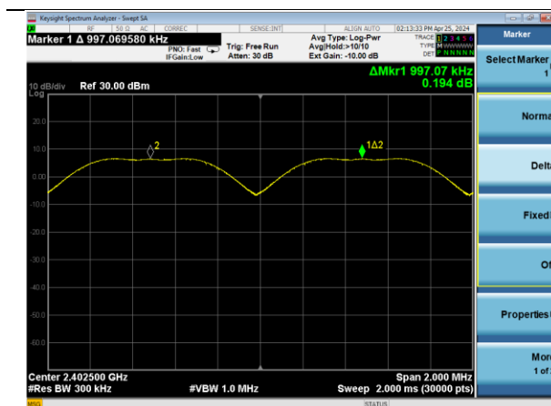
1DH5 | 997.1 kHz
