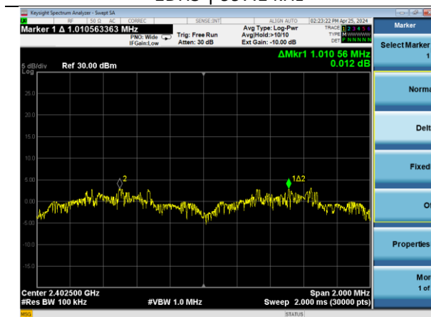
3DH5 | 1.011 MHz
