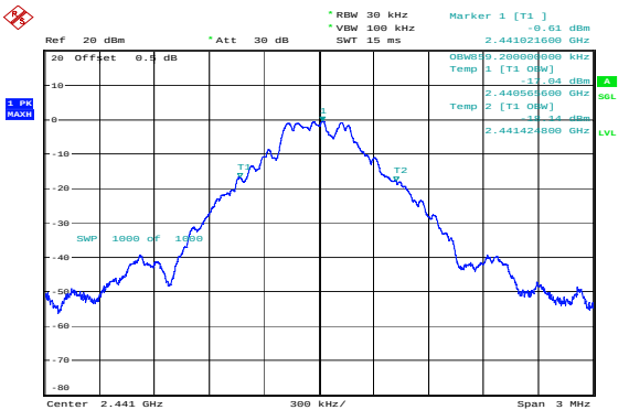
GFSK_Middle 0.859MHz
