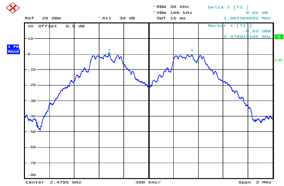
GFSK_High 1.002MHz
