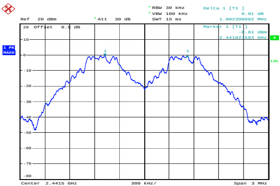
GFSK_Middle 1.002MHz
