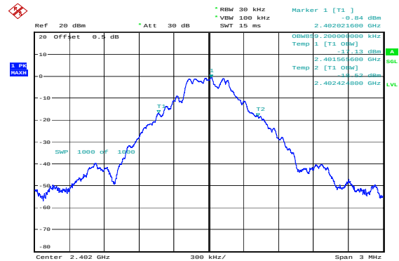
GFSK_Low 0.859MHz
