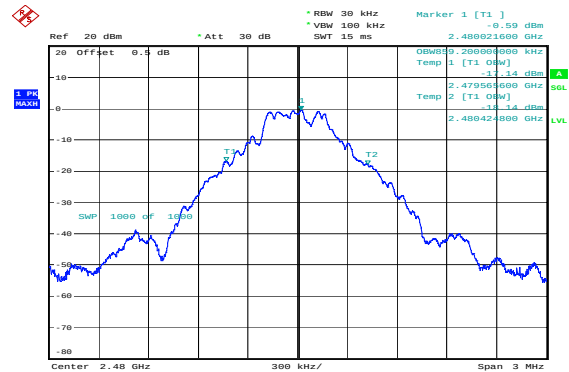
GFSK_High 0.859MHz
