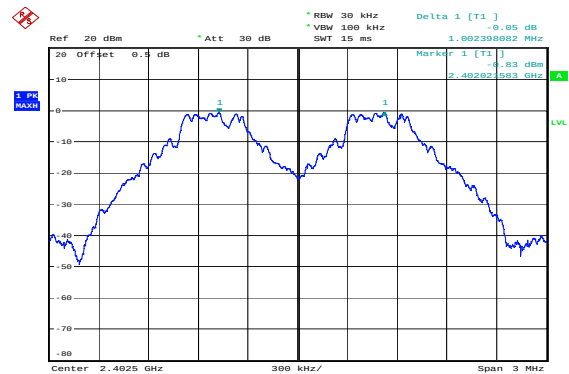
GFSK_Low 1.002MHz
