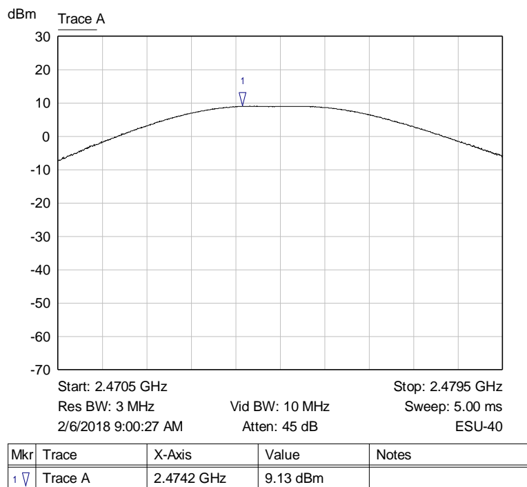
Graph 8: Highest Channel Output Power Plot (2475)
