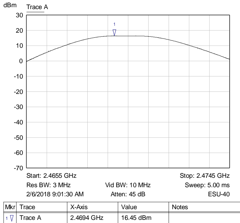
Graph 7: Channel 24 Output Power Plot (2470 MHz)
