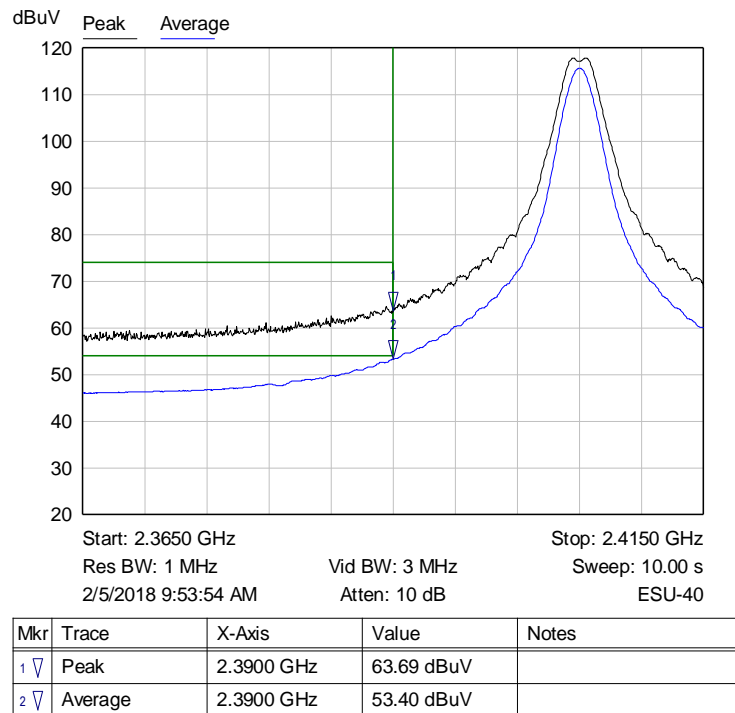
Graph 12: Radiated Channel 11 Lower Band Edge Plot (2405 MHz)
