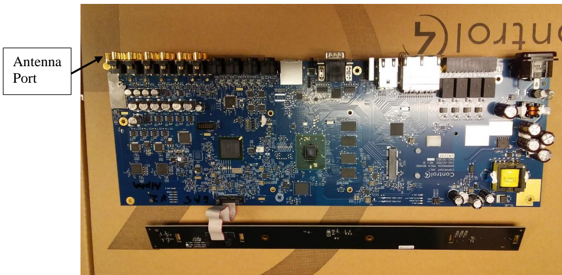
Photograph 11 – View of the Top Side of the PCB
