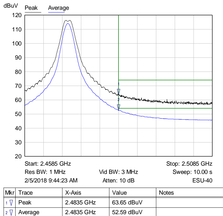
Graph 13: Radiated Channel 24 Upper Band Edge Plot (2470 MHz)
