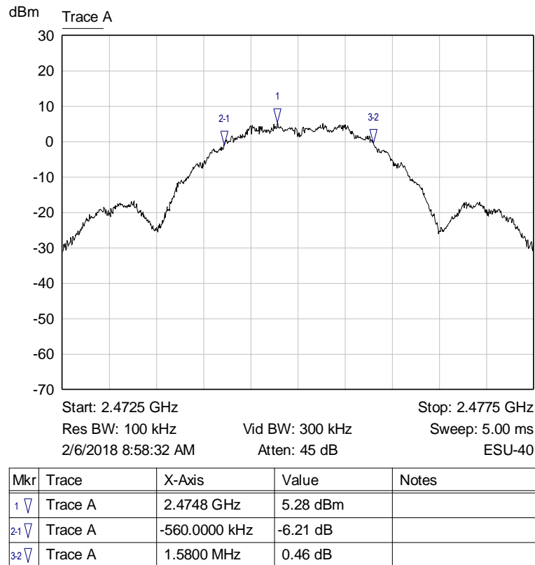
Graph 4: Highest Channel Bandwidth (2475 MHz)
