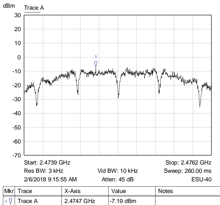
Graph 18: Highest Channel 3 kHz PSD Plot (2475 MHz)
