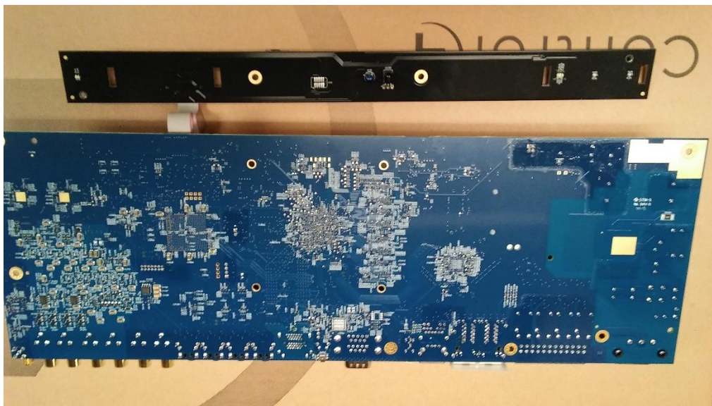
Photograph 12 – View of the Bottom Side of the PCB
