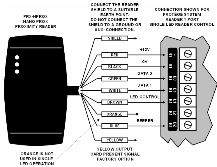
Figure 2 - Single LED Connection
