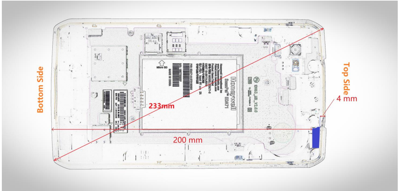
Back view
