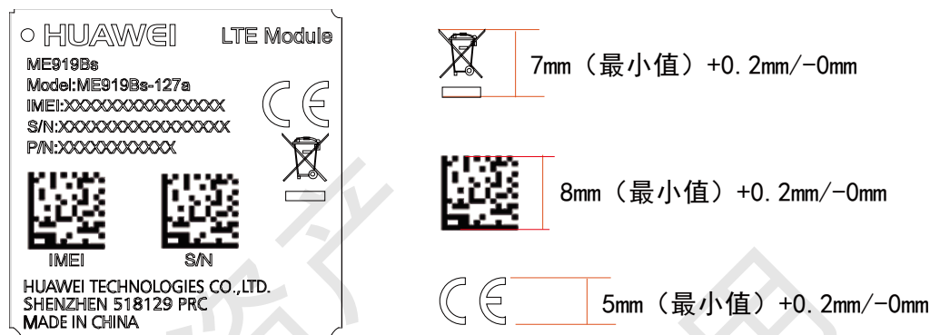
Figure 6-8 ME919Bs-127a Label
