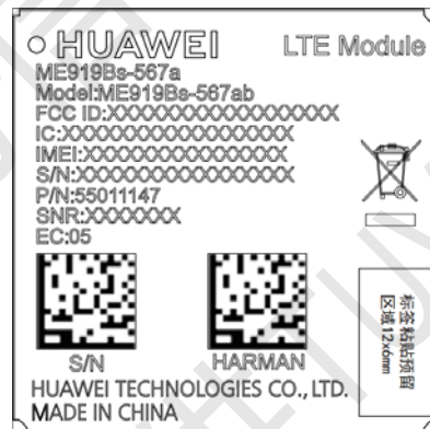
Figure 6-11 ME919Bs-567ab Label
