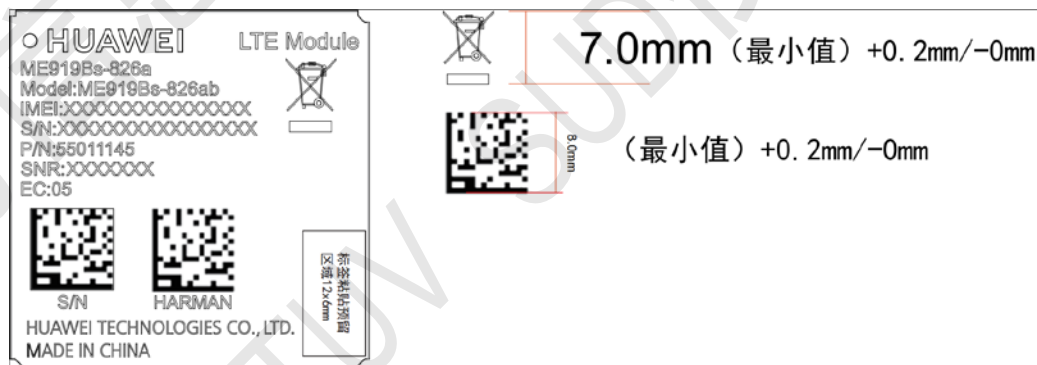
Figure 6-15 ME919Bs-826ab Label
