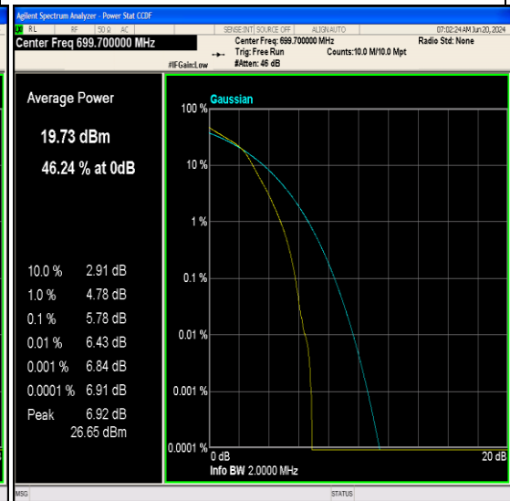
Band12-1.4MHz-16QAM-23017-6RB#0-PASS
