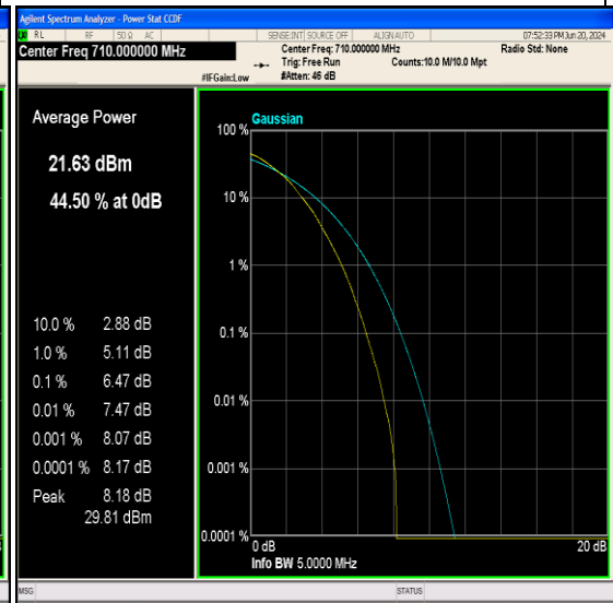
Band17-5MHz-64QAM-23790-25RB#0-PASS
