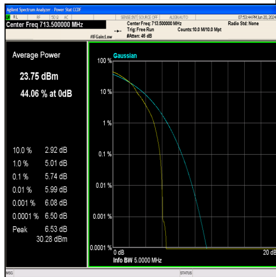
Band17-5MHz-64QAM-23825-1RB#0-PASS
