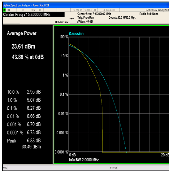
Band12-1.4MHz-64QAM-23173-1RB#0-PASS
