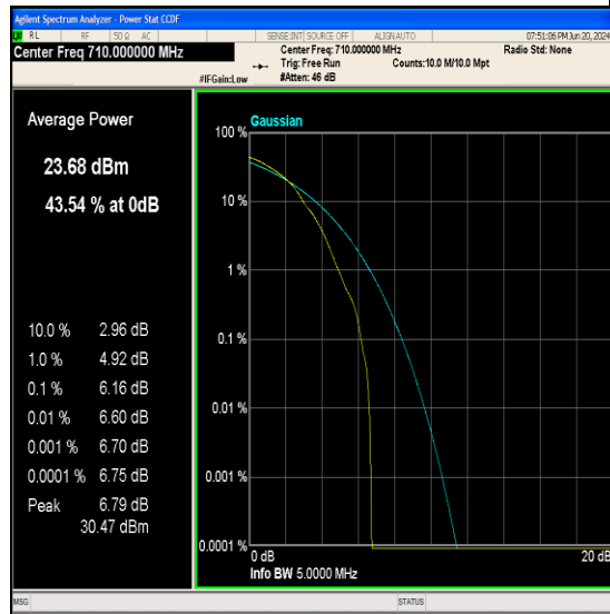
Band17-5MHz-64QAM-23790-1RB#0-PASS
