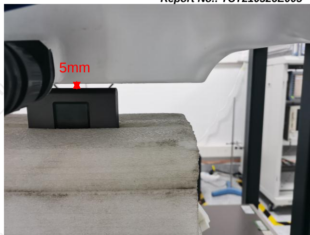
Hotspot Bottom(5mm)
