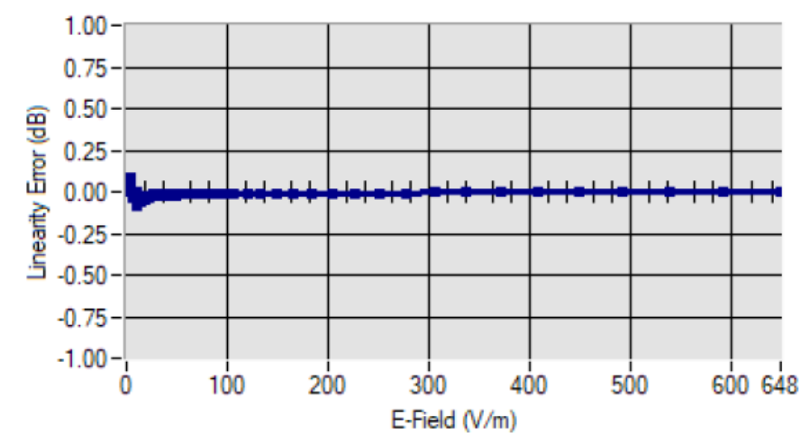
Linearity
