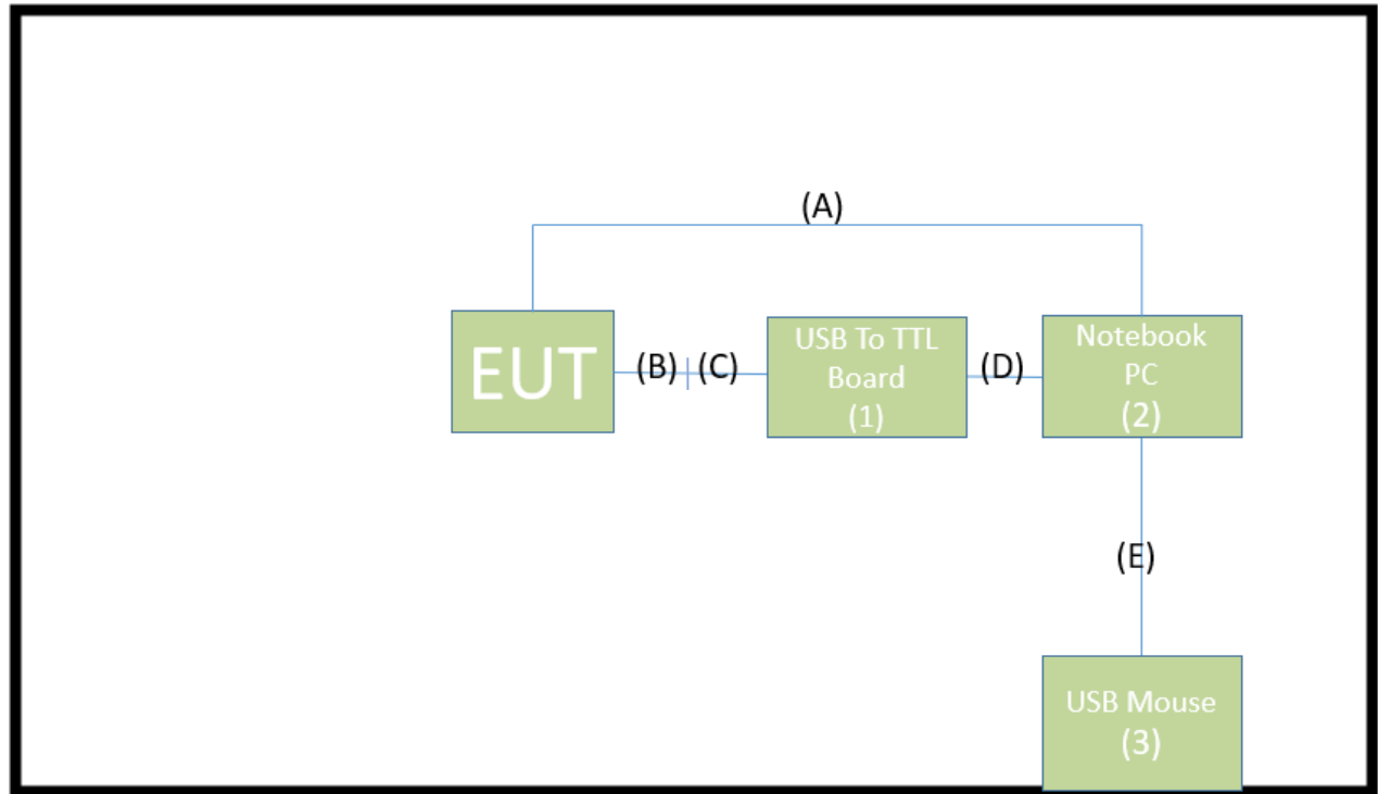
Connection Diagram
