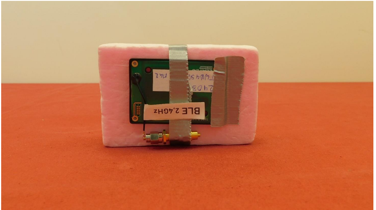
Picture 13: EUT position Z
