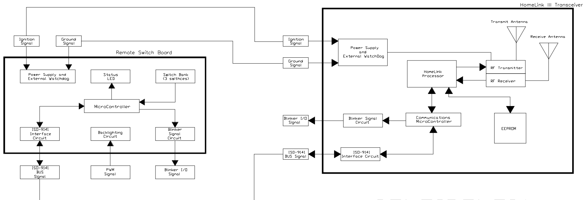
HomeLink III with remote switchboard (on the ISO9141 BUS) block diagram.
