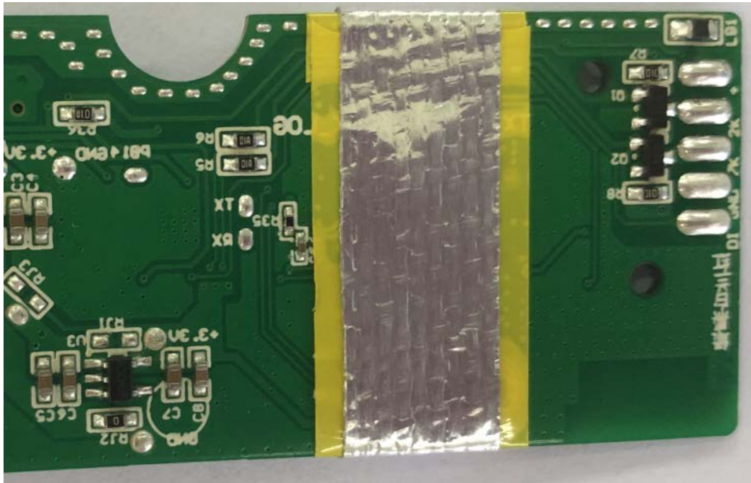
FIGURE 8 CYNC DIRECT CONNECTED OUTDOOR PREMIUM LIGHT STRIP (32FT.) (M/N: CLEDSTR36LCDODP) DEBUG1 BACK
