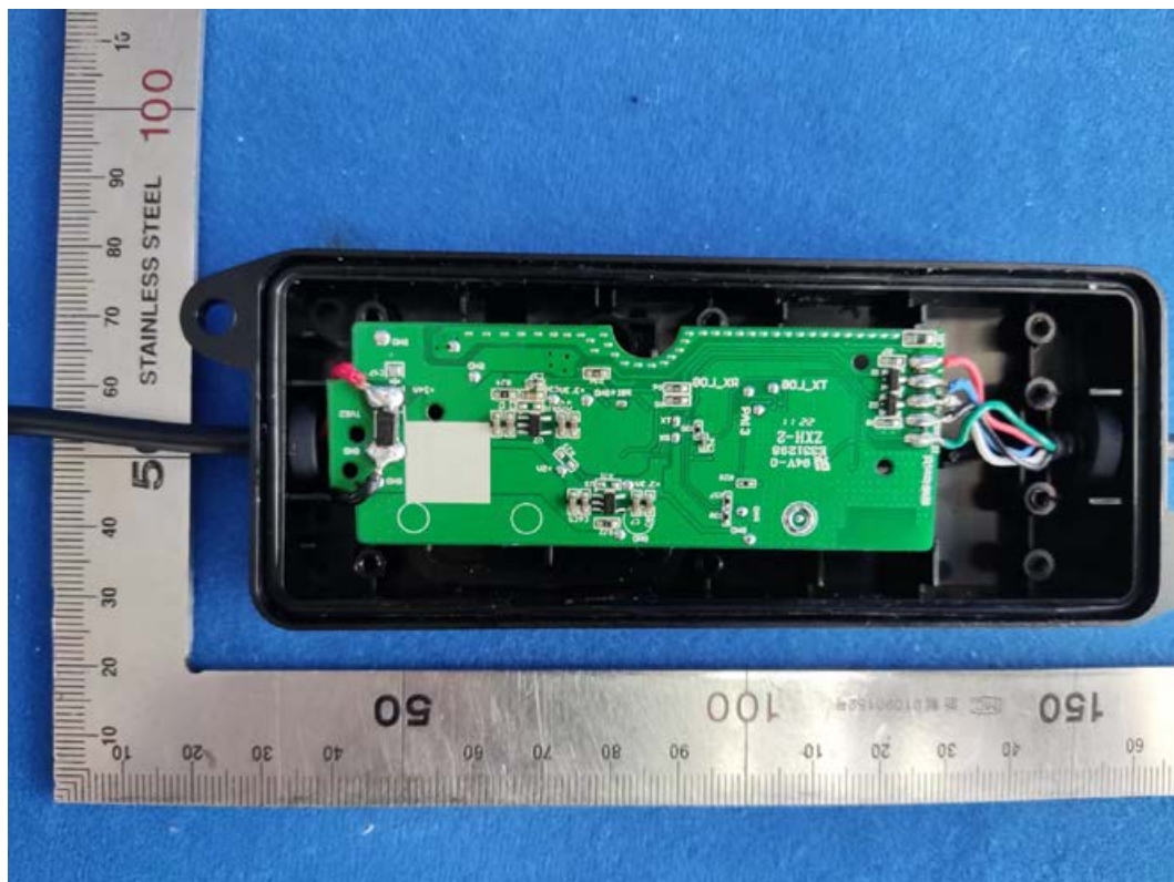
FIGURE 2 CYNC DIRECT CONNECTED OUTDOOR PREMIUM LIGHT STRIP (32FT.) (M/N: CLEDSTR36LCDODP) MAIN BOARD FRONT
