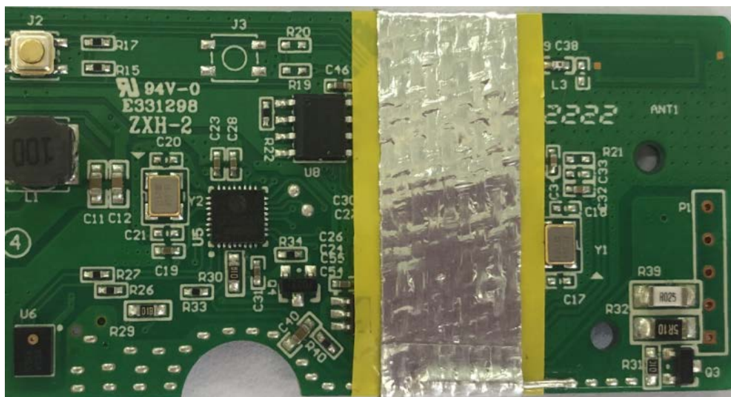
FIGURE 8 CYNC DIRECT CONNECTED OUTDOOR PREMIUM LIGHT STRIP (32FT.) (M/N: CLEDSTR36LCDODP) DEBUG1 BACK
