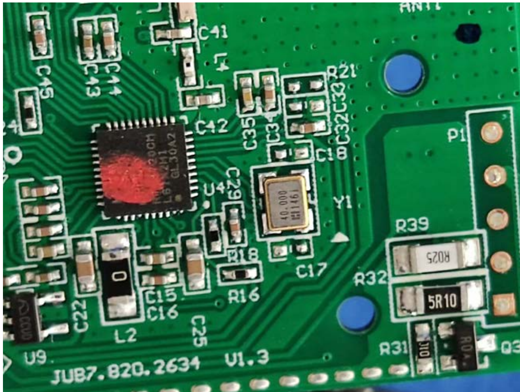
FIGURE 6 CYNC DIRECT CONNECTED OUTDOOR PREMIUM LIGHT STRIP (32FT.) (M/N: CLEDSTR36LCDODP) ANTENNA
