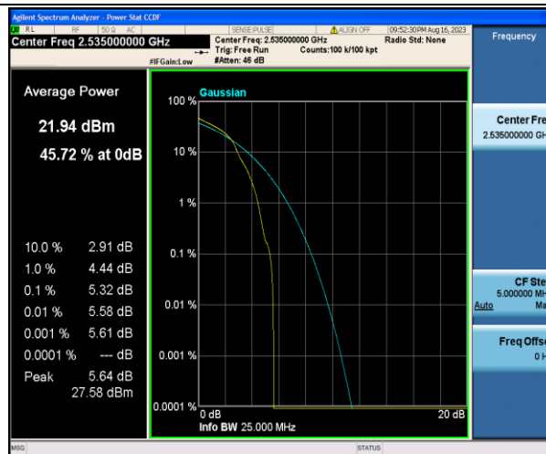
Band7-15MHz-16QAM-21100-1RB#0-PASS
