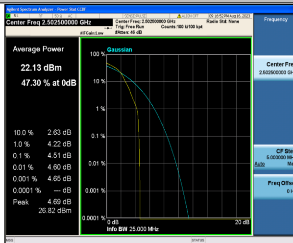
Band7-5MHz-16QAM-20775-1RB#0-PASS
