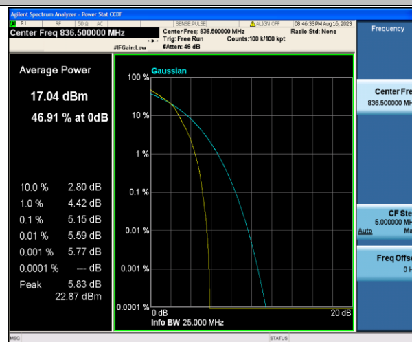
Band5-5MHz-16QAM-20525-25RB#0-PASS
