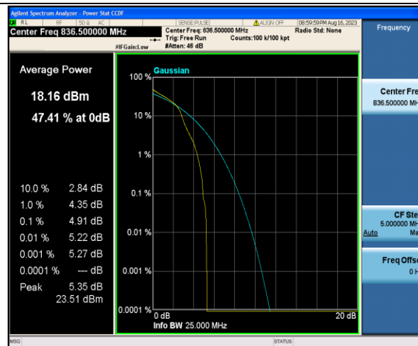
Band5-10MHz-16QAM-20525-1RB#0-PASS
