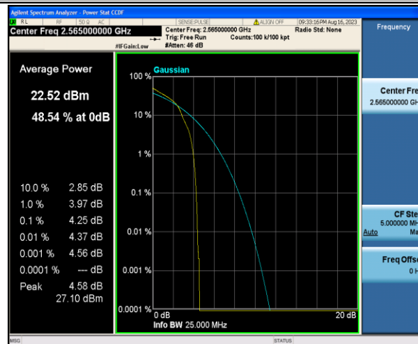
Band7-10MHz-16QAM-21400-1RB#0-PASS
