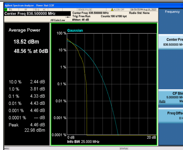
Band5-10MHz-QPSK-20525-1RB#0-PASS
