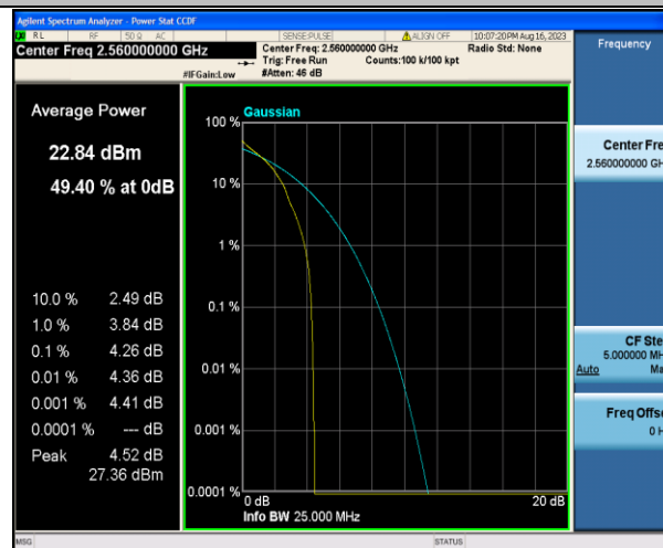
Band7-20MHz-QPSK-21350-1RB#0-PASS
