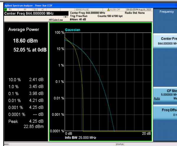
Band5-10MHz-QPSK-20600-1RB#0-PASS
