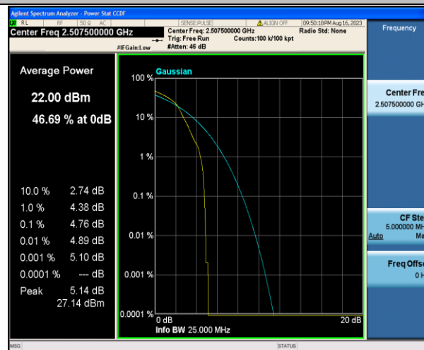
Band7-15MHz-16QAM-20825-1RB#0-PASS
