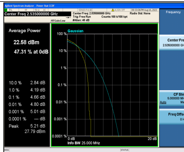
Band7-10MHz-16QAM-21100-1RB#0-PASS
