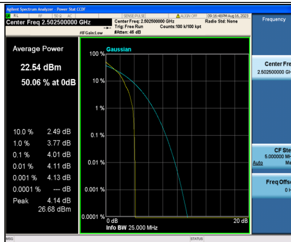
Band7-5MHz-QPSK-20775-1RB#0-PASS
