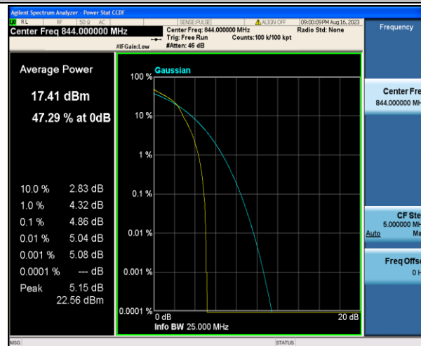
Band5-10MHz-16QAM-20600-1RB#0-PASS
