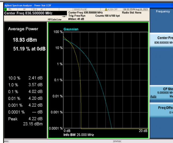
Band5-3MHz-QPSK-20525-1RB#0-PASS
