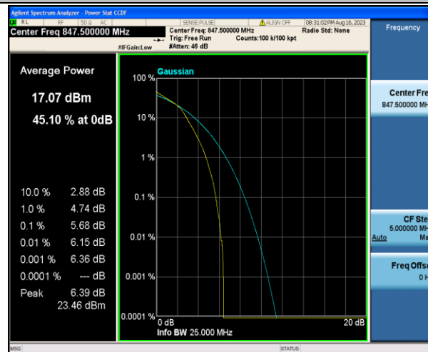
Band5-3MHz-16QAM-20635-15RB#0-PASS
