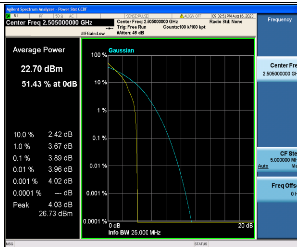
Band7-10MHz-QPSK-20800-1RB#0-PASS
