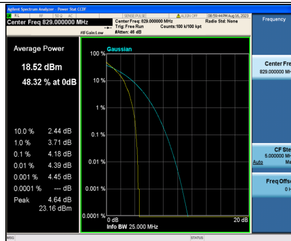
Band5-10MHz-QPSK-20450-1RB#0-PASS
