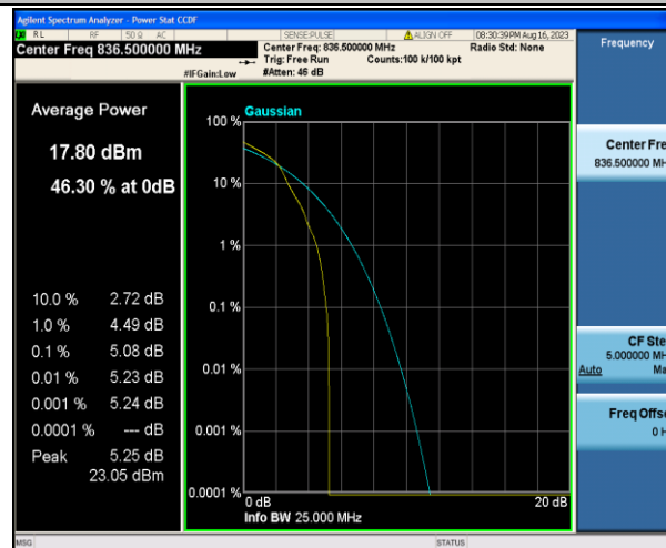
Band5-3MHz-16QAM-20525-1RB#0-PASS
