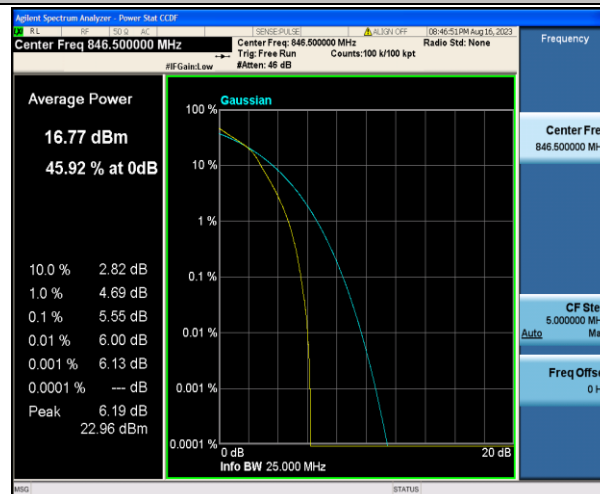
Band5-5MHz-16QAM-20625-25RB#0-PASS
