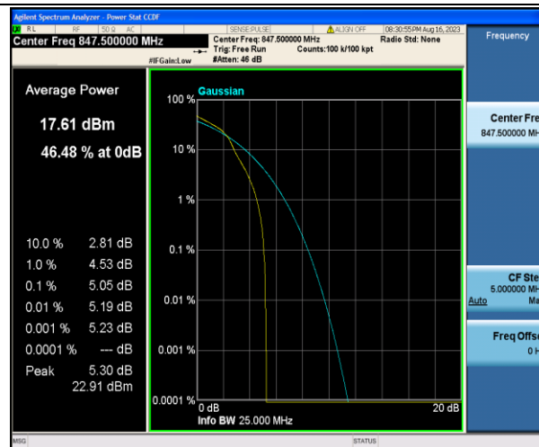
Band5-3MHz-16QAM-20635-1RB#0-PASS
