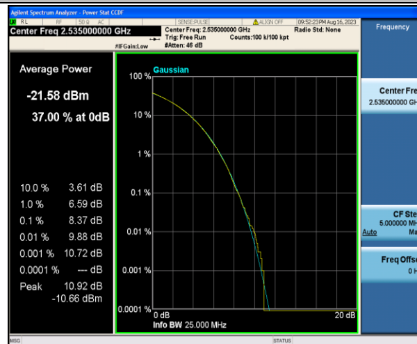
Band7-15MHz-QPSK-21100-1RB#0-PASS
