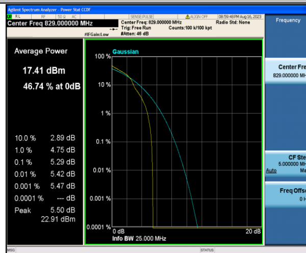
Band5-10MHz-16QAM-20450-1RB#0-PASS
