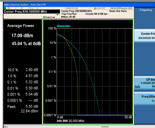
Band5-5MHz-16QAM-20525-1RB#0-PASS
