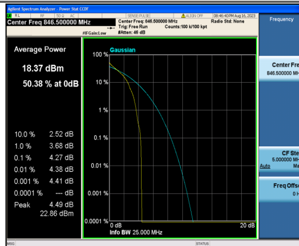
Band5-5MHz-QPSK-20625-1RB#0-PASS
