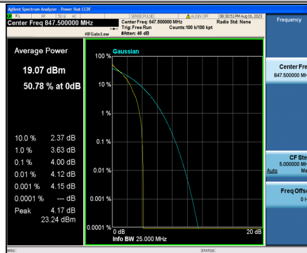
Band5-3MHz-QPSK-20635-1RB#0-PASS
