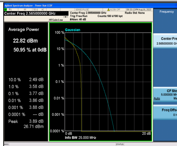
Band7-10MHz-QPSK-21400-1RB#0-PASS
