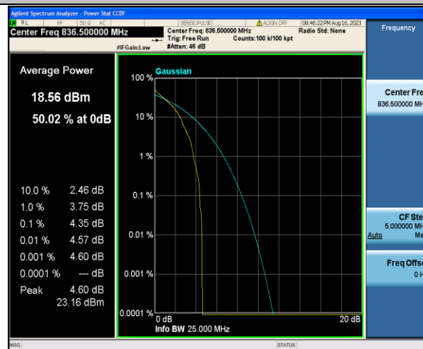
Band5-5MHz-QPSK-20525-1RB#0-PASS
