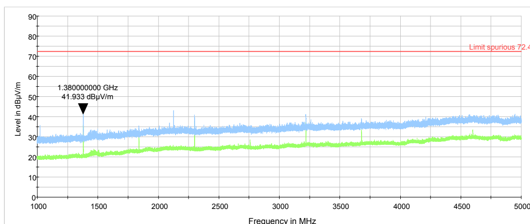
Plot 7.4.18 Radiated emission measurements in 1000 – 5000 MHz range
