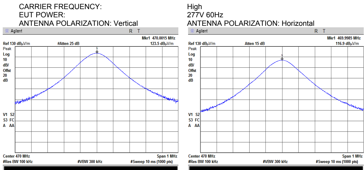
Plot 7.1.6 Transmitter carrier field strength at high frequency in vertical and horizontal antenna polarization
