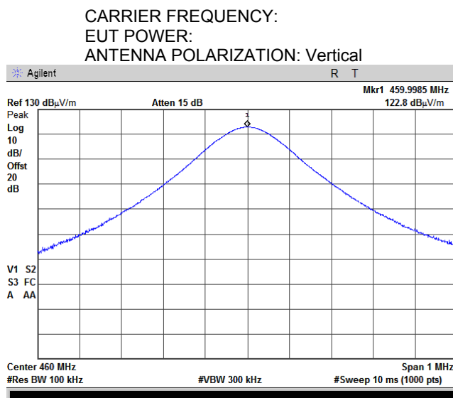
Plot 7.1.2 Transmitter carrier field strength at mid frequency in vertical and horizontal antenna polarization
