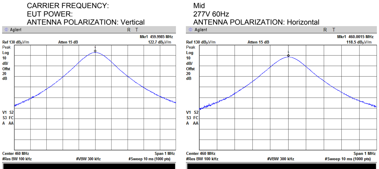
Plot 7.1.5 Transmitter carrier field strength at mid frequency in vertical and horizontal antenna polarization
