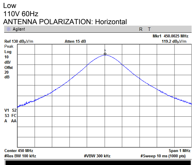
Plot 7.1.1 Transmitter carrier field strength at low frequency in vertical and horizontal antenna polarization
