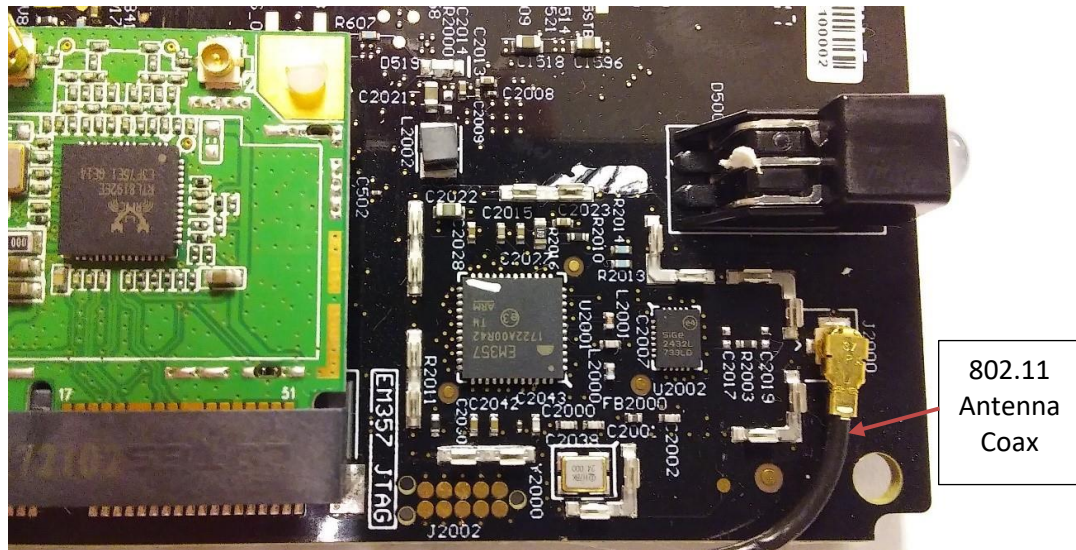
Photograph 3 – Back View of the EUT PCB
