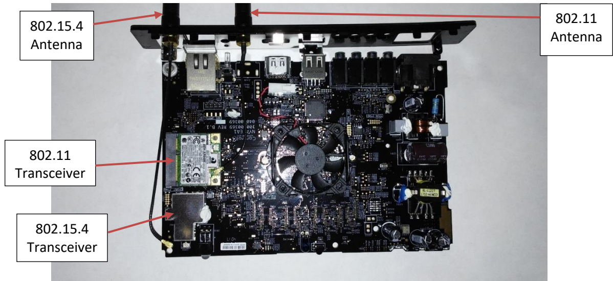
Photograph 1 – Top View of the PCB
