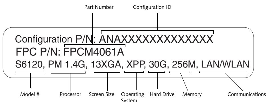
Figure 7-1 Configuration Label
