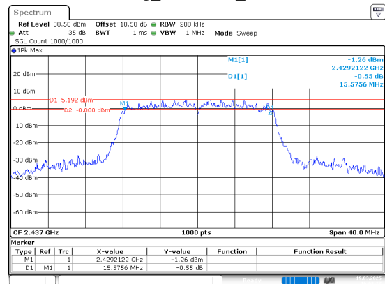
802.11g_2437MHz_Chain 0
