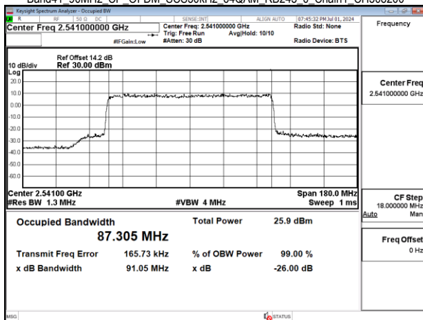
Band41_90MHz_CP_OFDM_SCS30kHz_64QAM_RB245_0_Chain1_CH508200
