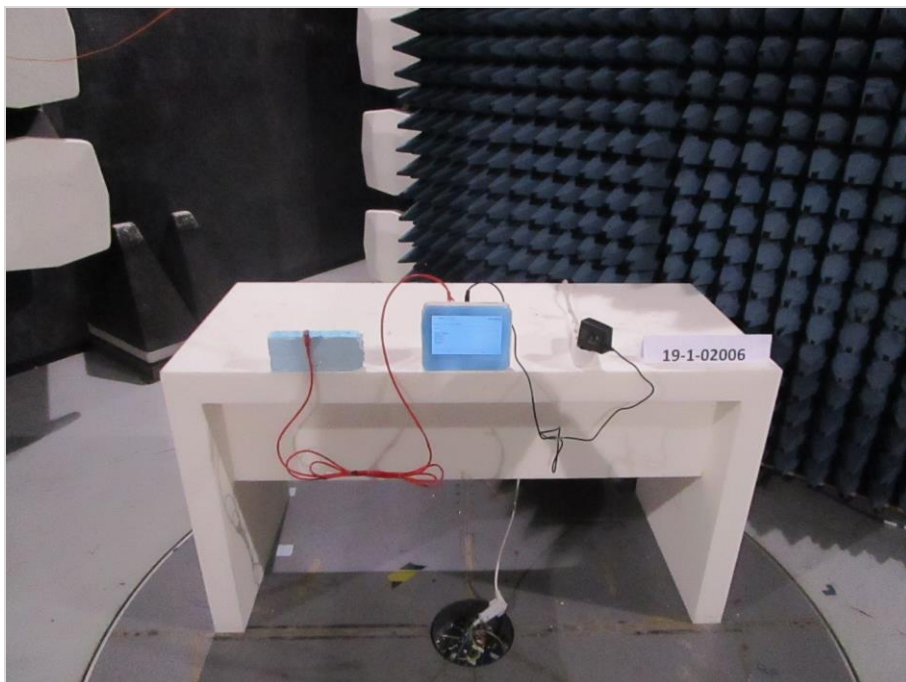
Photograph 6: EUT Test Setup in the semi anechoic chamber, Radiated interference field
