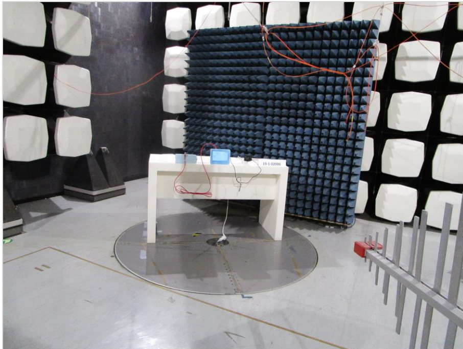
Photograph 5: EUT Test Setup in the semi anechoic chamber, Radiated interference field
