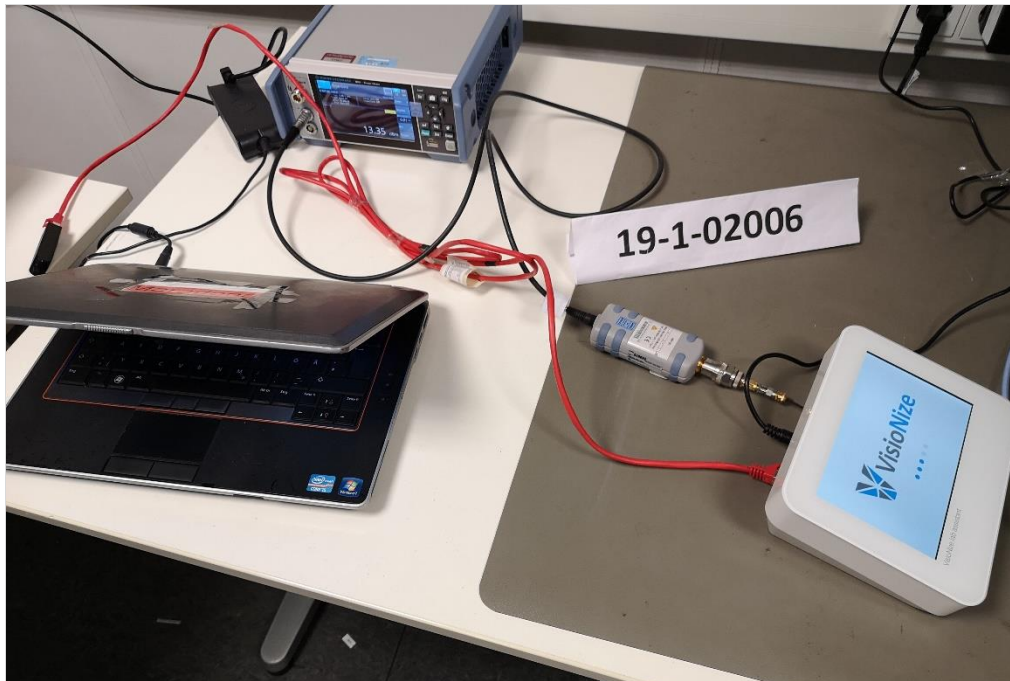
Photograph 7: Conducted test setup in the Radio Lab
