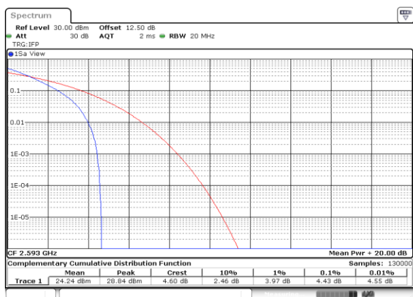
LTE Band 41 / 20MHz / 64QAM
