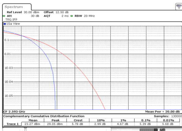
LTE Band 41 / 20MHz / 256QAM
