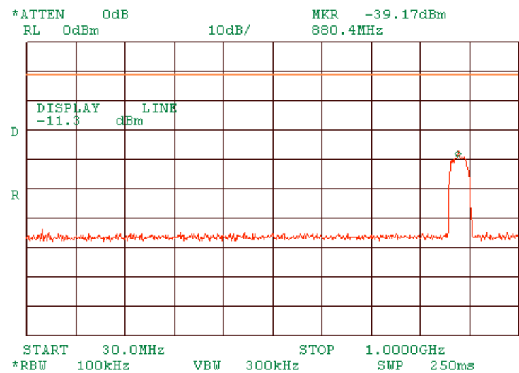
Plot 1.9.10 Spurious emission measurements in 30 - 1000 MHz range at low carrier frequency DSSS
