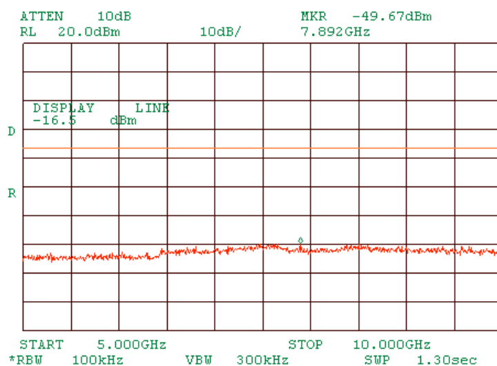
Plot 1.7.58 Spurious emission measurements in 5000 - 10000 MHz range at mid carrier frequency OFDM
