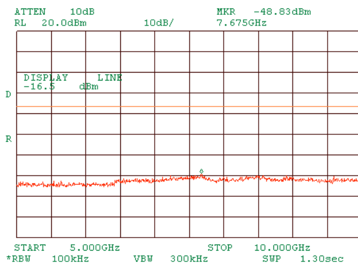
Plot 1.7.57 Spurious emission measurements in 5000 - 10000 MHz range at low carrier frequency OFDM
