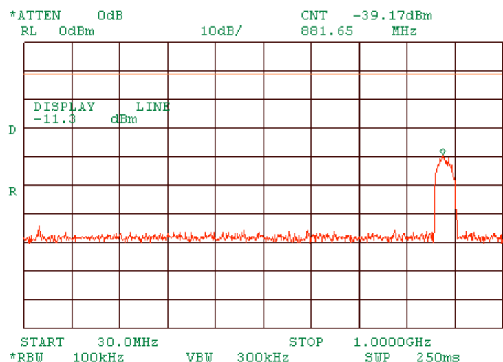
Plot 1.9.14 Spurious emission measurements in 30 - 1000 MHz range at high carrier frequency DSSS
