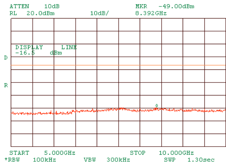
Plot 1.7.59 Spurious emission measurements in 5000 - 10000 MHz range at high carrier frequency OFDM
