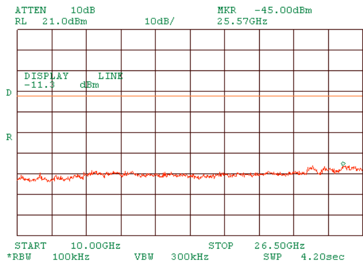
Plot 1.9.27 Spurious emission measurements in 10000 - 26500 MHz range at high carrier frequency DSSS
