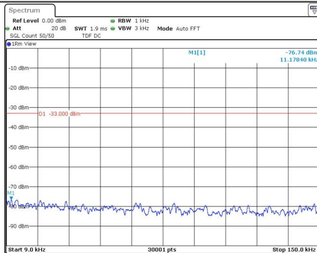
Band5-4182-1-0.009~0.15MHz
