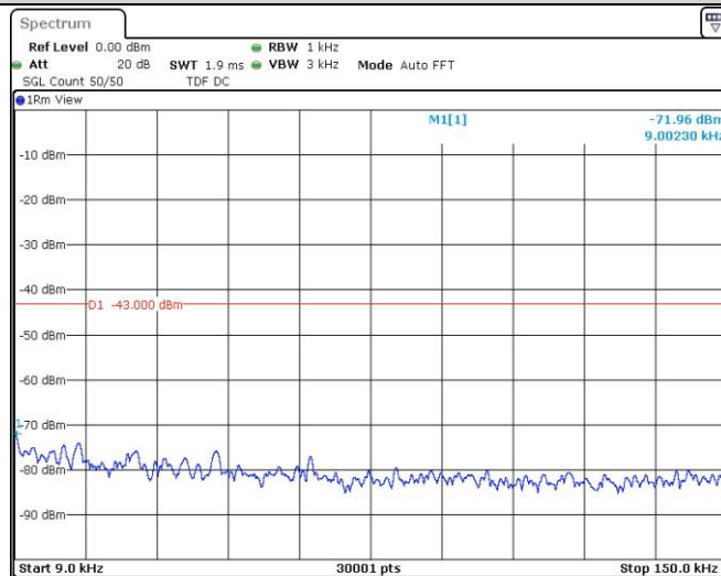
Band4-1312-3-0.009~0.15MHz
