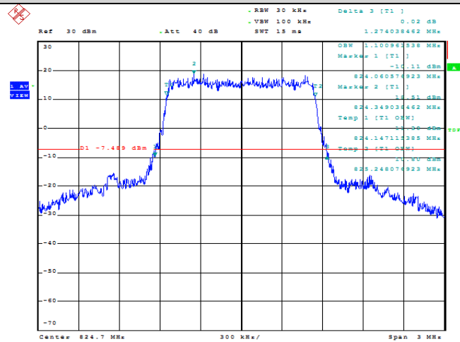
Band5-1.4MHz-QPSK-20407-6RB#0-1.101
