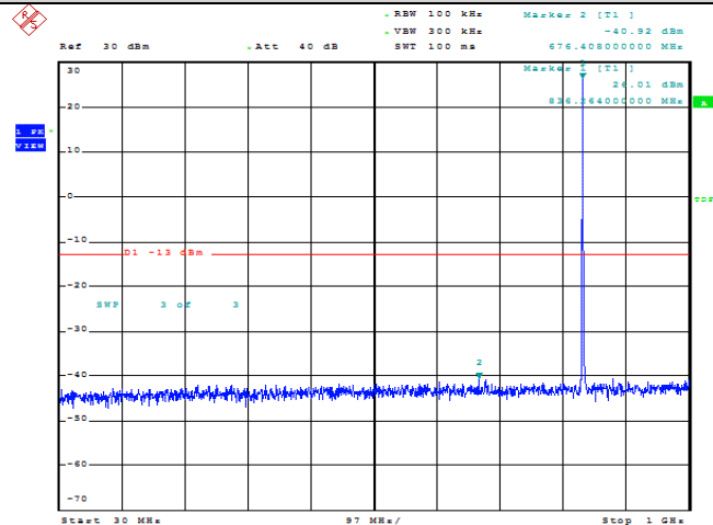
Band5-1.4MHz-QPSK-20525-1RB#0-Range1:30~1000MHz
