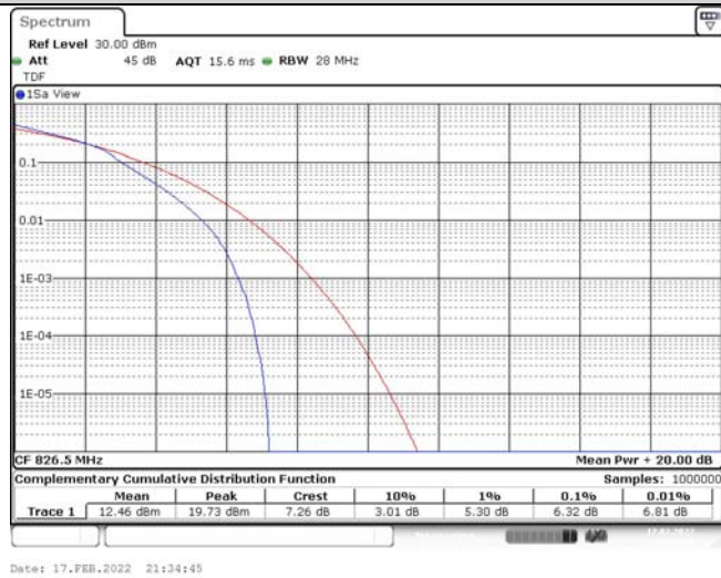
Band5-5MHz-16QAM-20525-1RB#0
