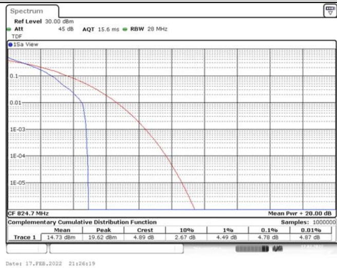
Band5-1.4MHz-QPSK-20407-6RB#0
