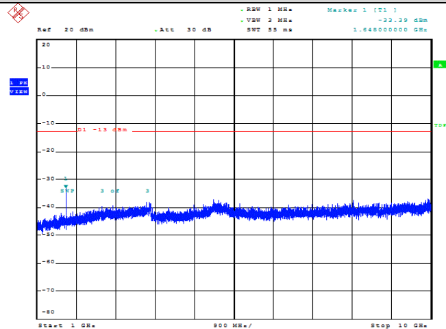
Band5-1.4MHz-QPSK-20407-1RB#0-Range2:1000~10000MHz
