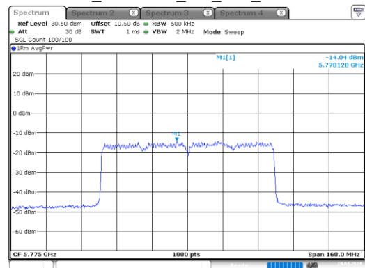
ax80_5775MHz_RU_Full_Chain 1
