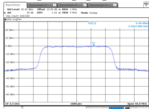
ax20_5200MHz_RU_Full_Chain 1
