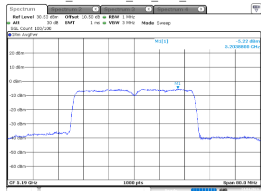
ax40_5190MHz_RU_Full_Chain 1
