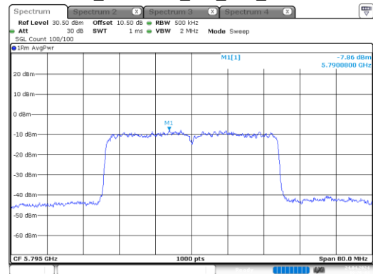
ax40_5795MHz_RU_Full_Chain 1
