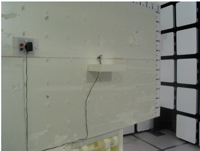
Picture 1 Spurious radiated emission measurement Bluetooth TX
