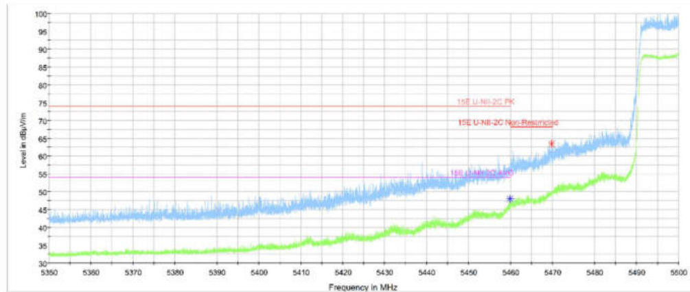
Fig. 31 Band Edges (802.11ax-HT40 , full RU, Ch102, 5510MHz, MIMO)
