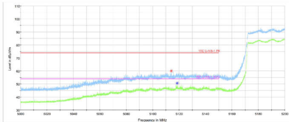
Fig. 37 Band Edges (802.11ax-HT160 , full RU, Ch50, 5250MHz, MIMO)
