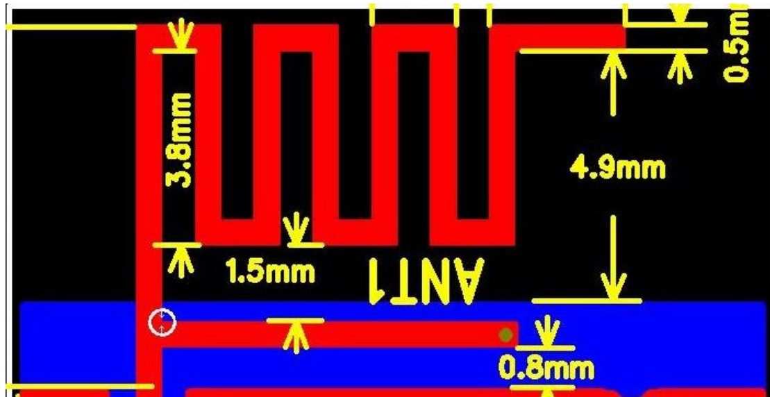
3-1 Normal Module Wiggles Antenna
