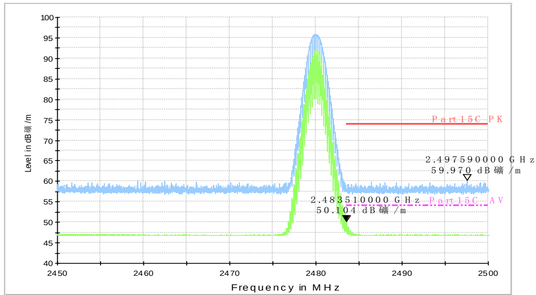
Fig.63. Radiated emission (Power): 8DPSK, high channel
