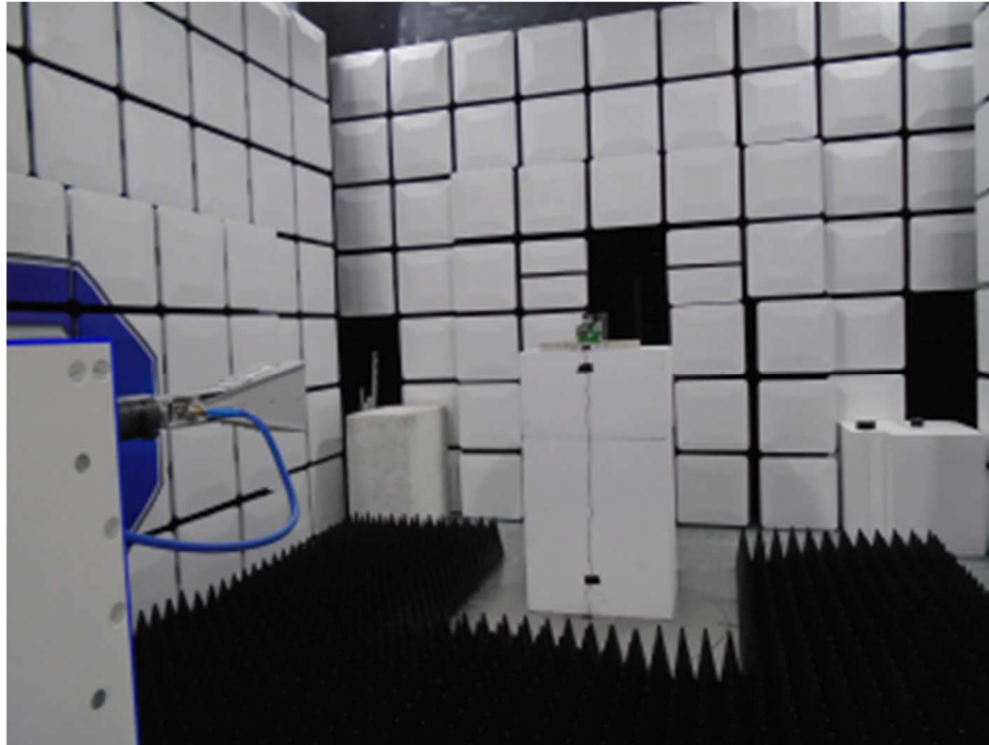
Figure 3 – Radiated Disturbance - 8 GHz to 18 GHz
